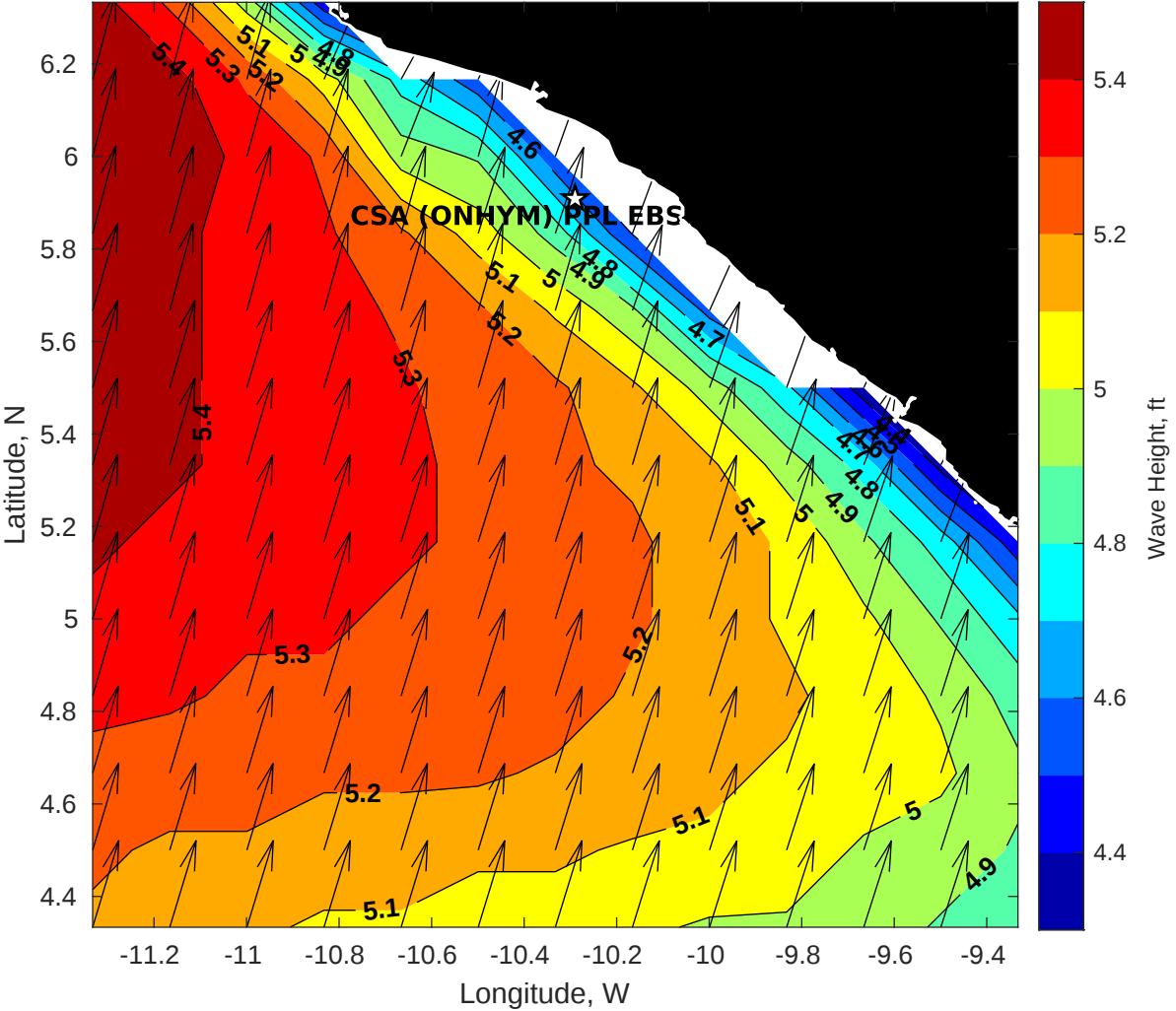
Wave Height (ft) for CSA (ONHYM) PPL EBS - Liberia at 06-Sep-2025 09:00:00
