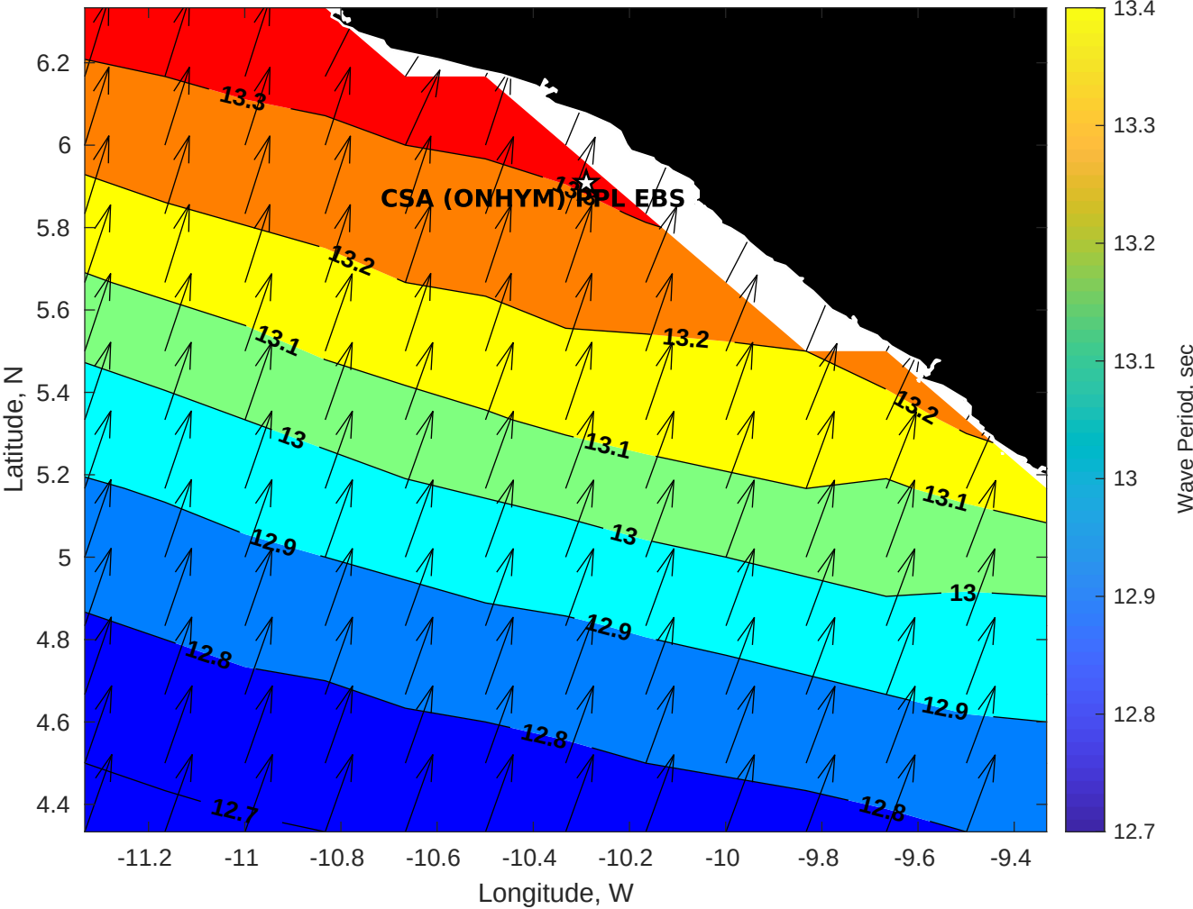
Wave Period (sec) for CSA (ONHYM) PPL EBS - Liberia at 06-Sep-2025 09:00:00
