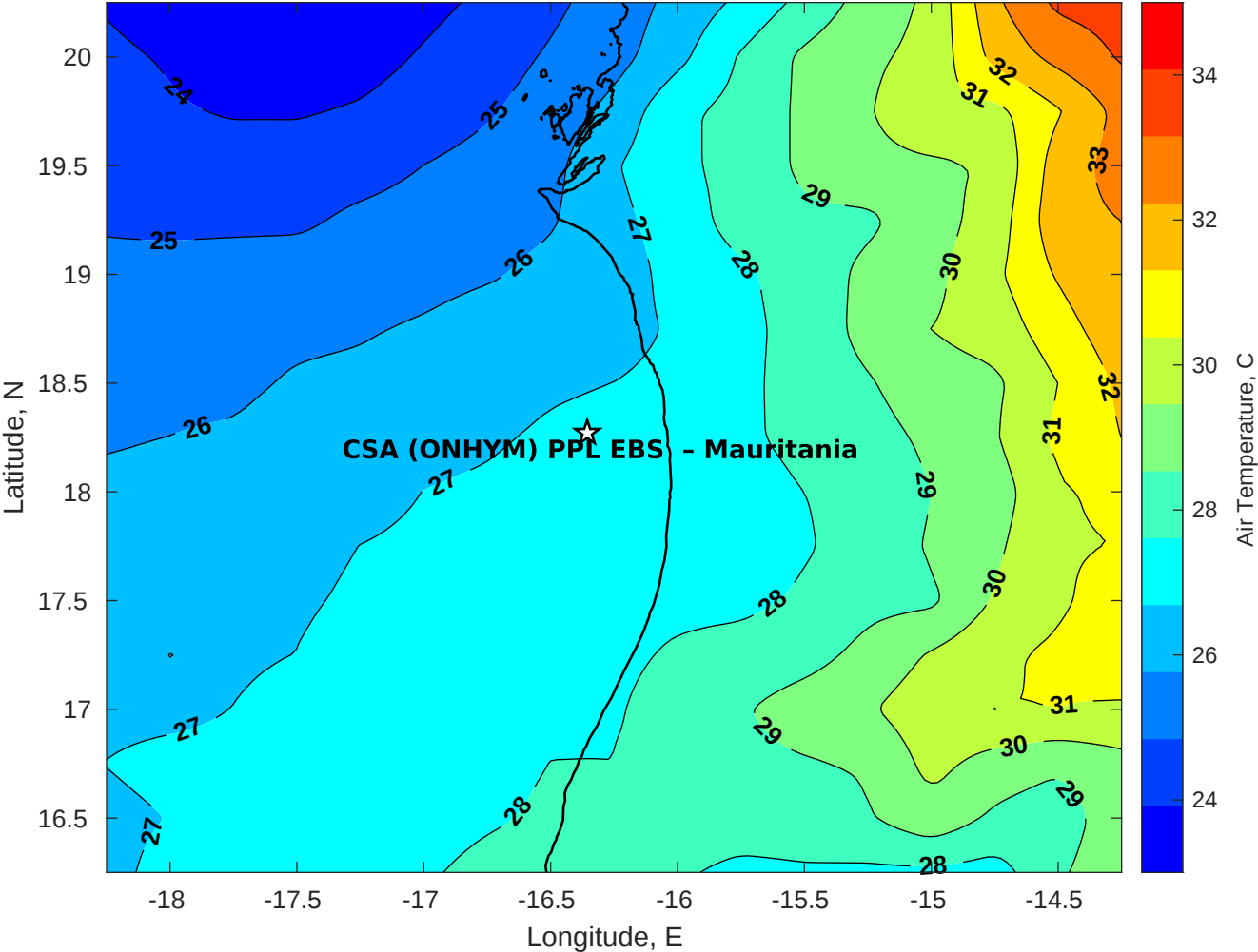
Air Temperature (C) for CSA (ONHYM) PPL EBS - Mauritania at 06-Sep-2025
