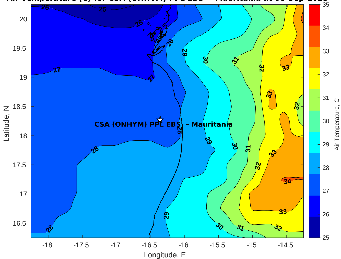
Air Temperature (C) for CSA (ONHYM) PPL EBS - Mauritania at 06-Sep-2025
