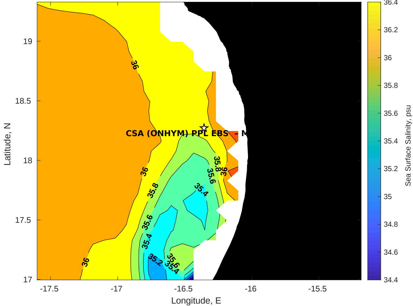
Surface Salinity for CSA (ONHYM) PPL EBS - Mauritania at 05-Sep-2025 00:00:00
