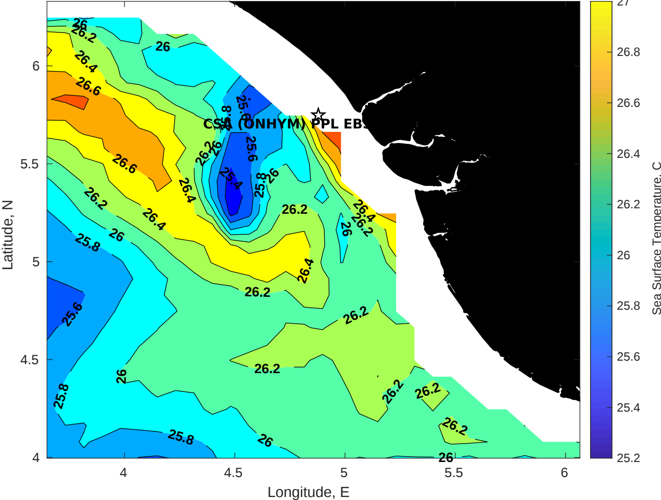
SST for CSA (ONHYM) PPL EBS - Nigeria at 05-Sep-2025 00:00:00
