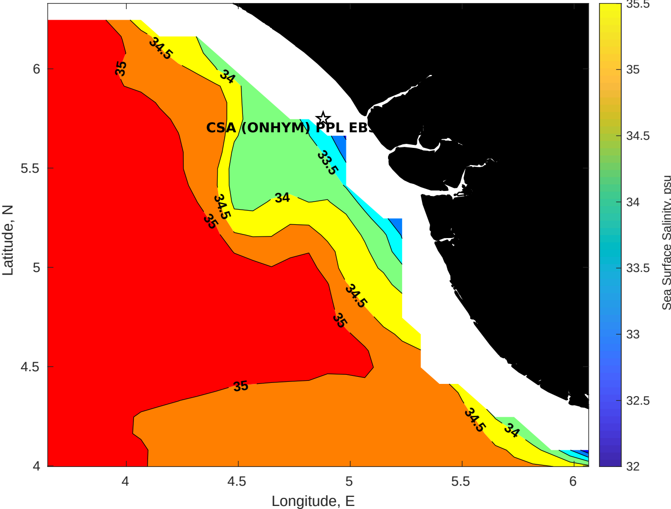
Surface Salinity for CSA (ONHYM) PPL EBS - Nigeria at 05-Sep-2025 00:00:00
