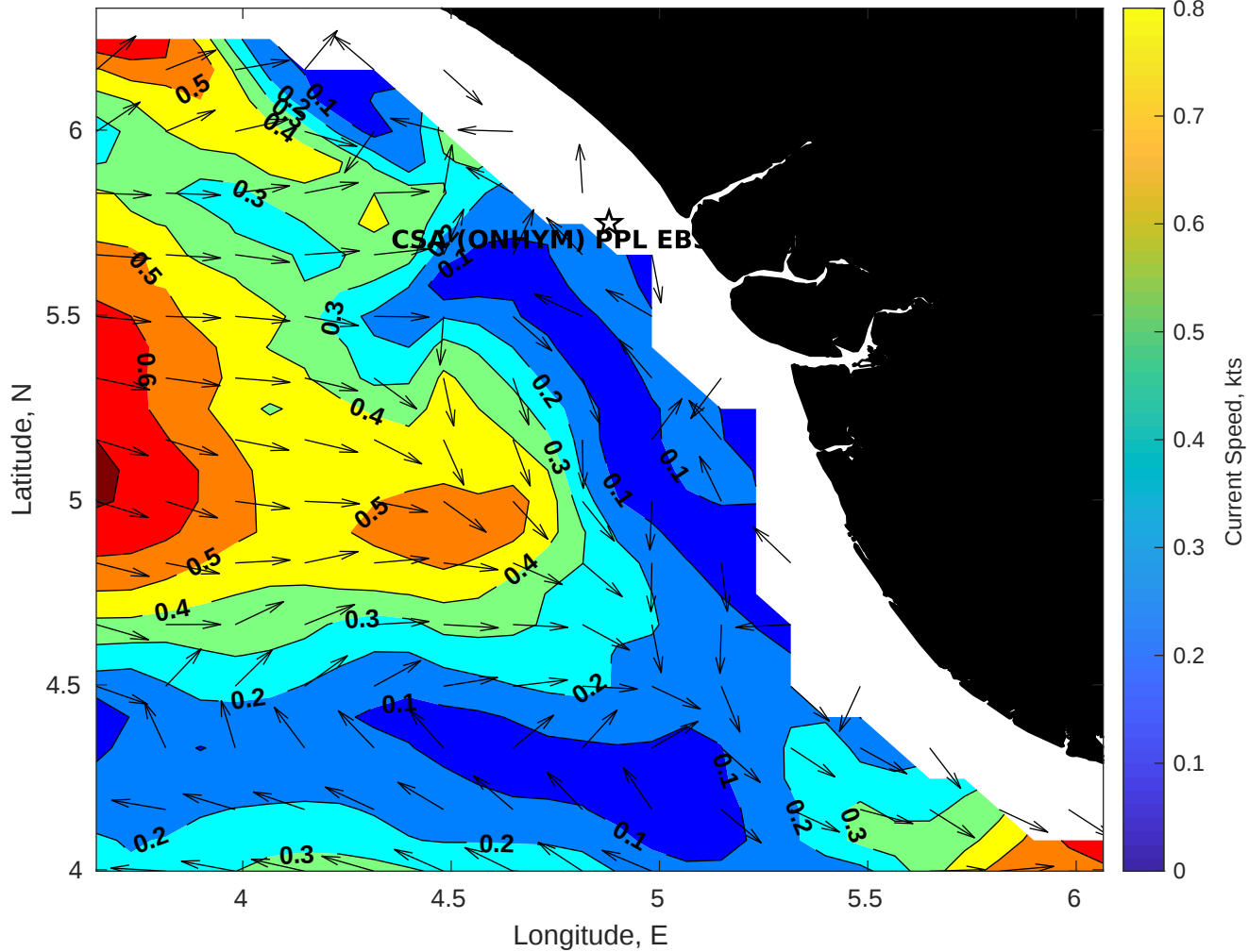
Surface Currents for CSA (ONHYM) PPL EBS - Nigeria at 05-Sep-2025 00:00:00
