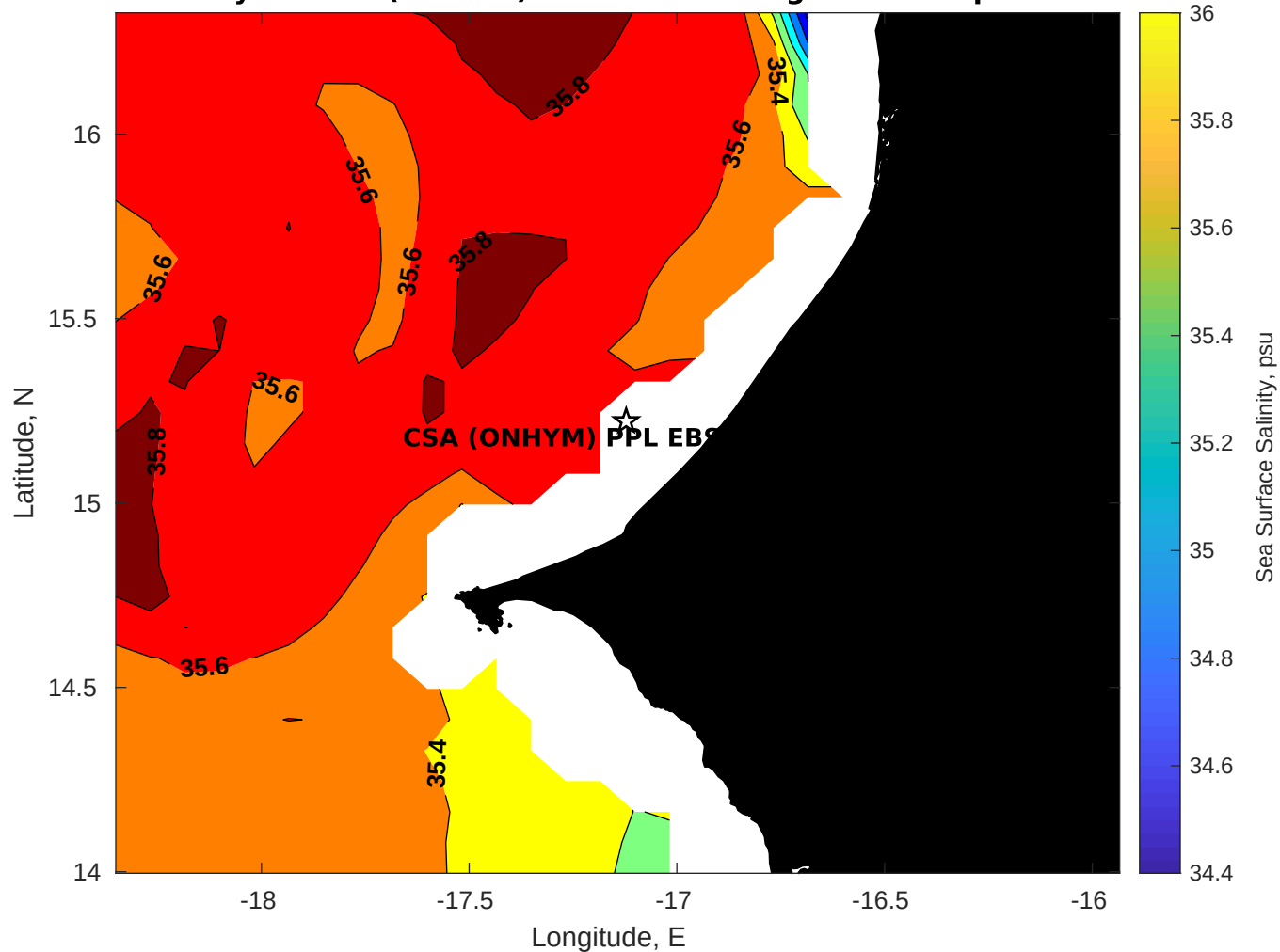
Surface Salinity for CSA (ONHYM) PPL EBS - Senegal at 05-Sep-2025 00:00:00
