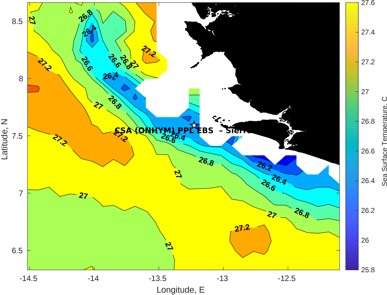
SST for CSA (ONHYM) PPL EBS - Sierra Leone at 05-Sep-2025 00:00:00
