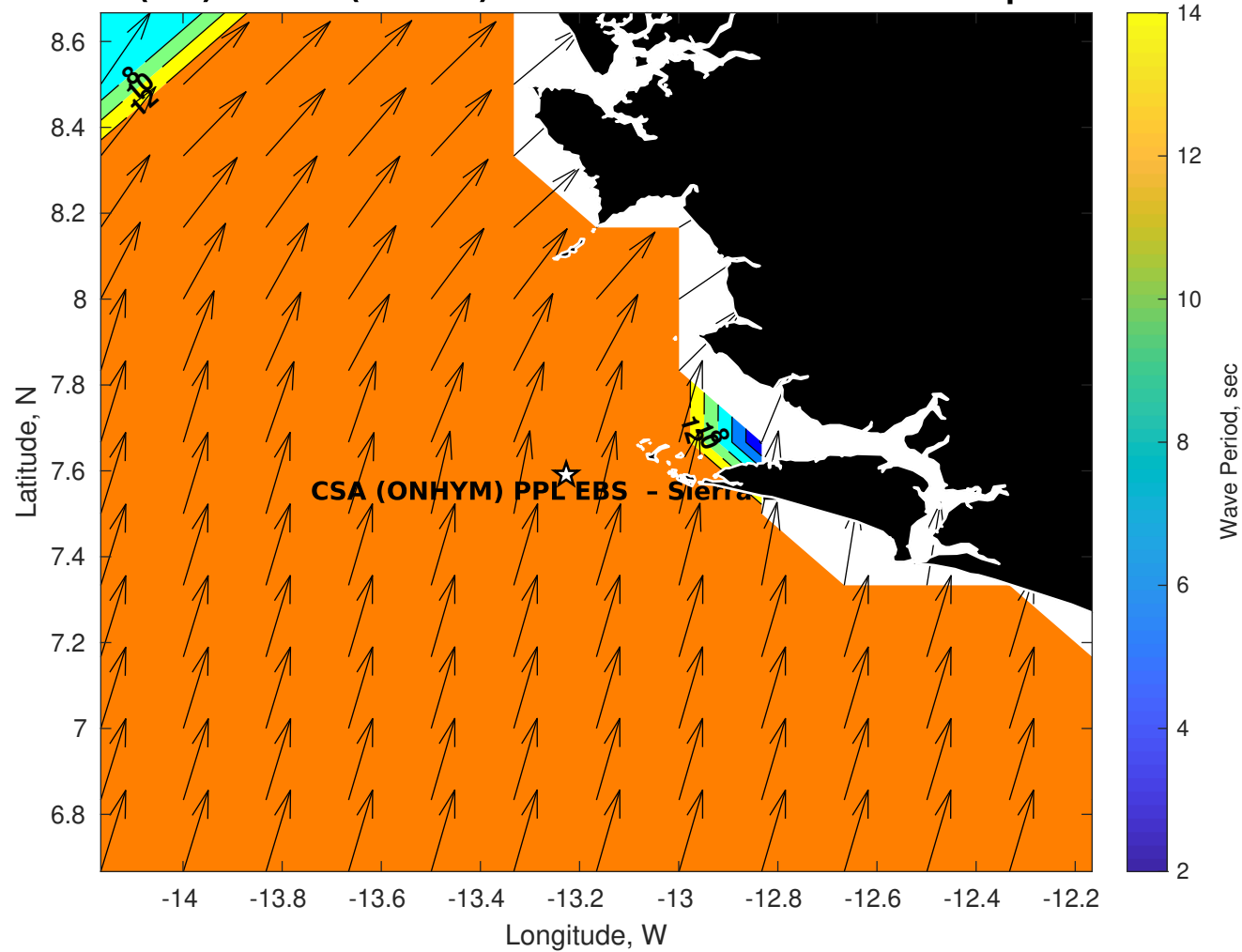
Wave Period (sec) for CSA (ONHYM) PPL EBS - Sierra Leone at 06-Sep-2025 09:00:00
