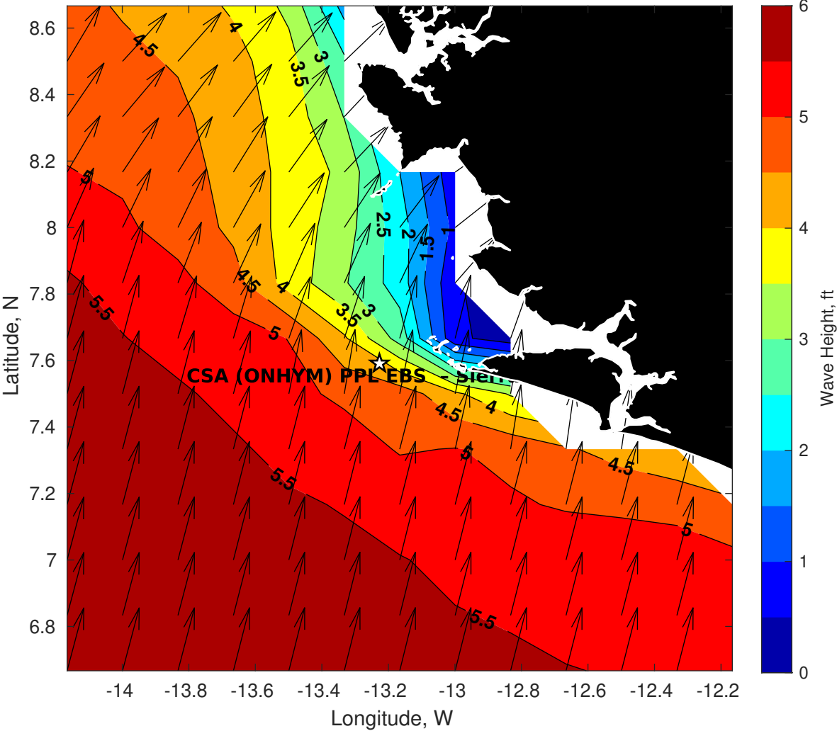
Wave Height (ft) for CSA (ONHYM) PPL EBS - Sierra Leone at 06-Sep-2025 09:00:00
