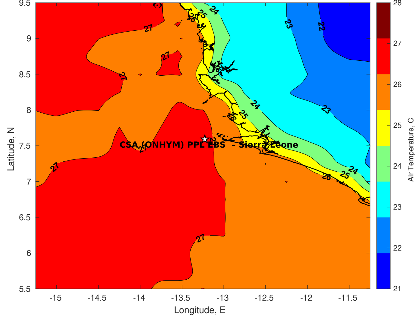
Air Temperature (C) for CSA (ONHYM) PPL EBS - Sierra Leone at 06-Sep-2025
