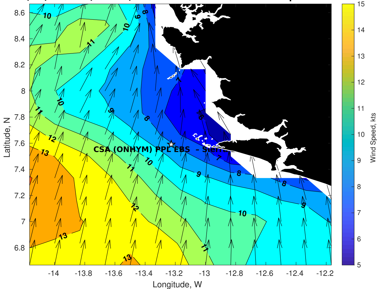
Winds (kts) for CSA (ONHYM) PPL EBS - Sierra Leone at 06-Sep-2025 09:00:00
