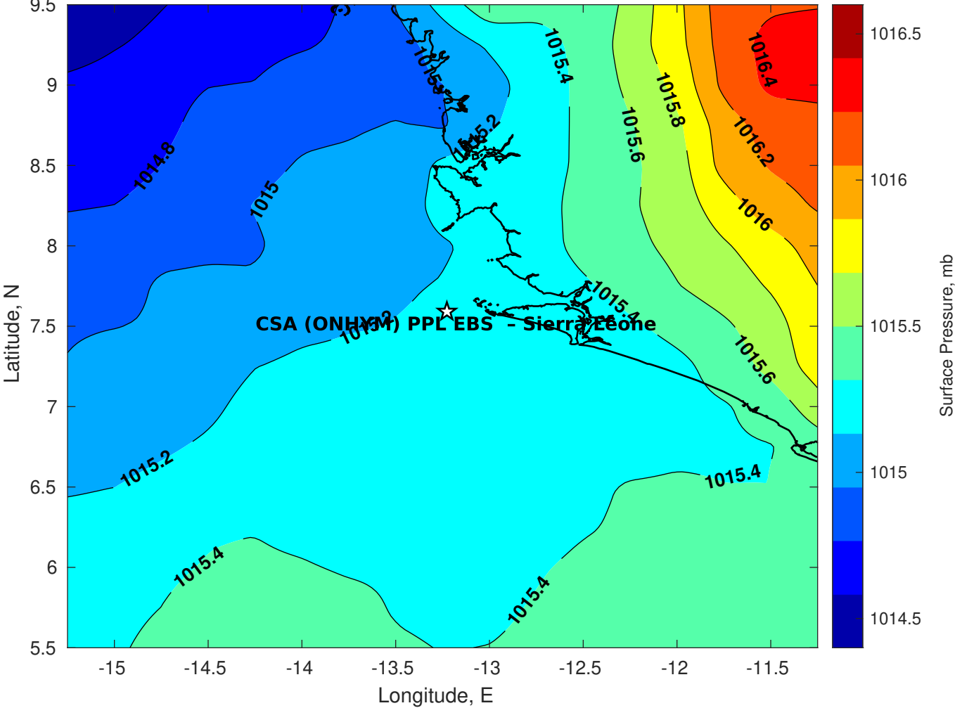
Surface Pressure (mb) for CSA (ONHYM) PPL EBS - Sierra Leone at 07-Sep-2025 00:00:00
