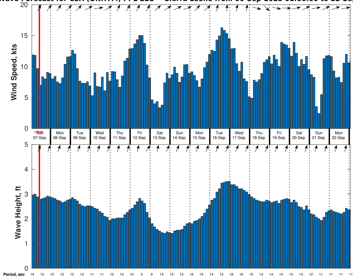
Wind & Wave Forecast for CSA (ONHYM) PPL EBS - Sierra Leone from 06-Sep-2025 01:00:00 to 22-Sep-2025 01:00:00
