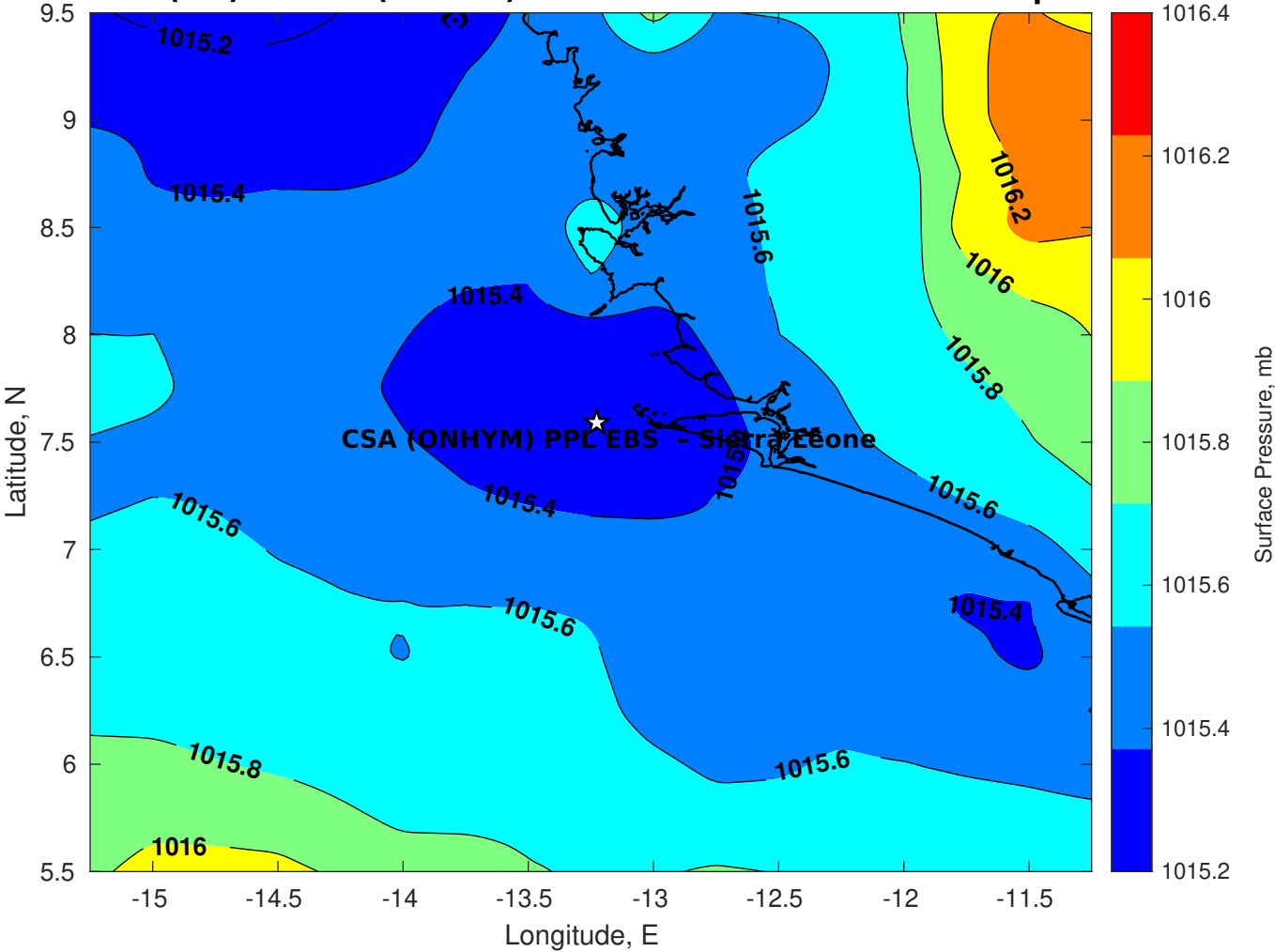
Surface Pressure (mb) for CSA (ONHYM) PPL EBS - Sierra Leone at 08-Sep-2025 00:00:00
