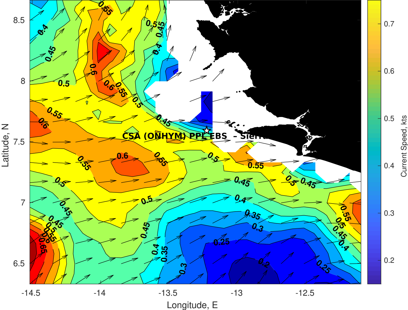
Surface Currents for CSA (ONHYM) PPL EBS - Sierra Leone at 05-Sep-2025 00:00:00
