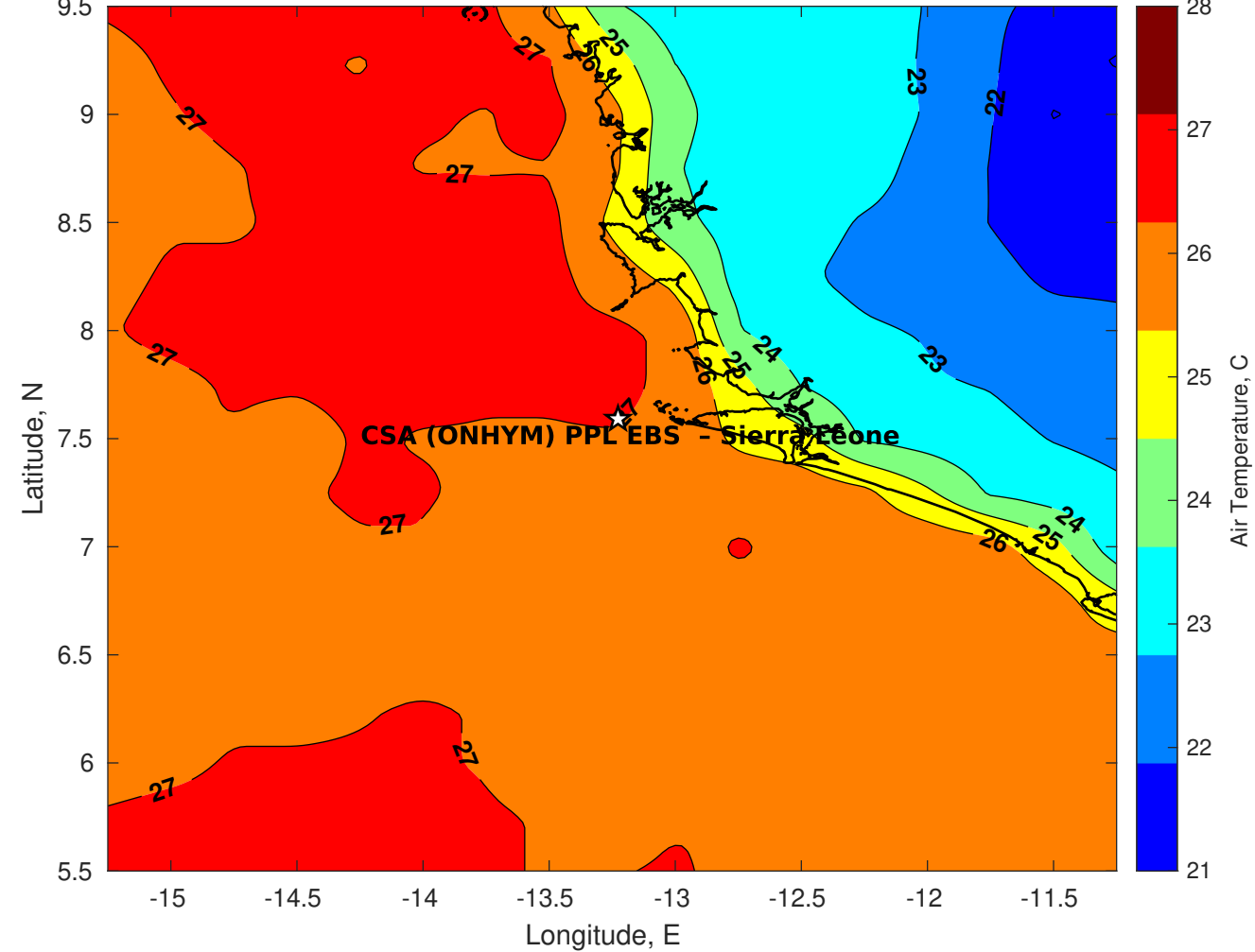
Air Temperature (C) for CSA (ONHYM) PPL EBS - Sierra Leone at 06-Sep-2025
