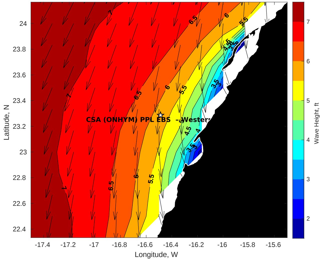
Wave Height (ft) for CSA (ONHYM) PPL EBS - Western Sahara at 06-Sep-2025 09:00:00
