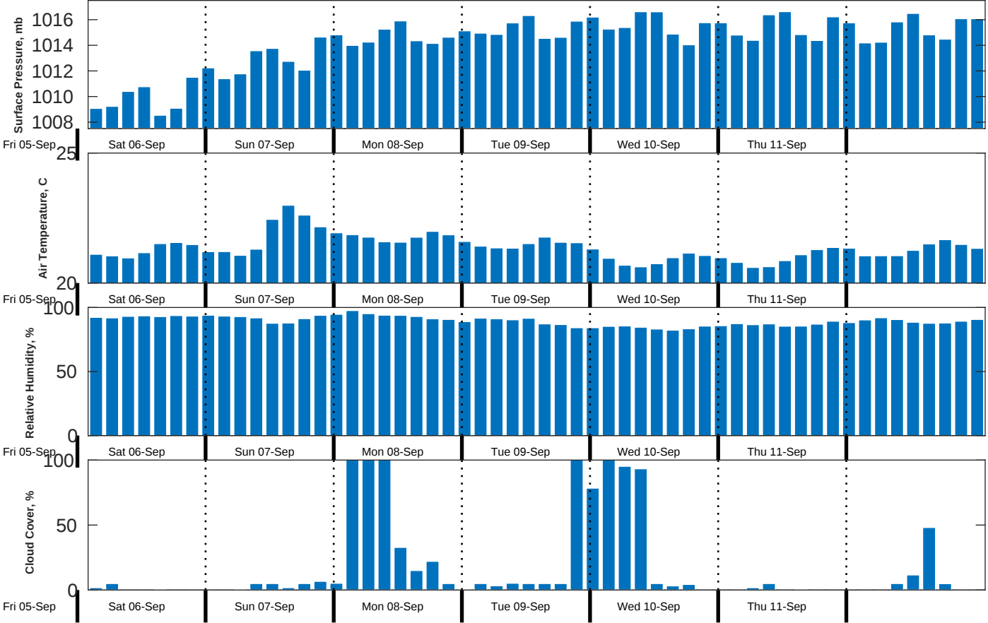
Met Forecast for CSA (ONHYM) PPL EBS - Western Sahara from 06-Sep-2025 00:00:00 to 13-Sep-2025 00:00:00
