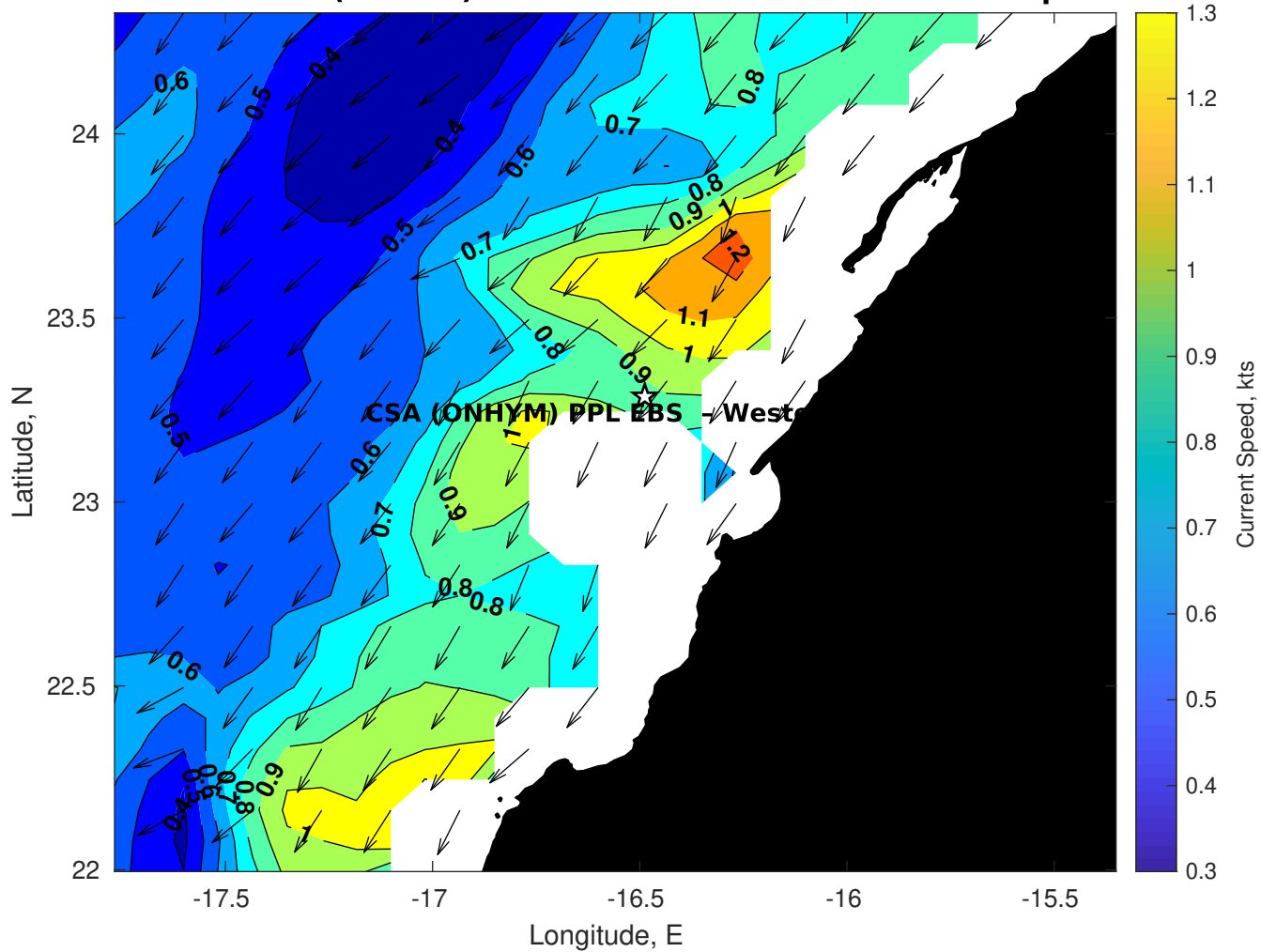
Surface Currents for CSA (ONHYM) PPL EBS - Western Sahara at 05-Sep-2025 00:00:00
