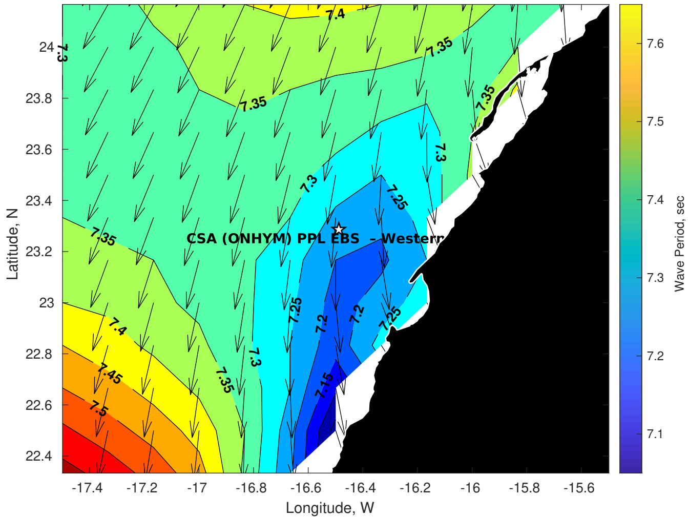
Wave Period (sec) for CSA (ONHYM) PPL EBS - Western Sahara at 06-Sep-2025 09:00:00
