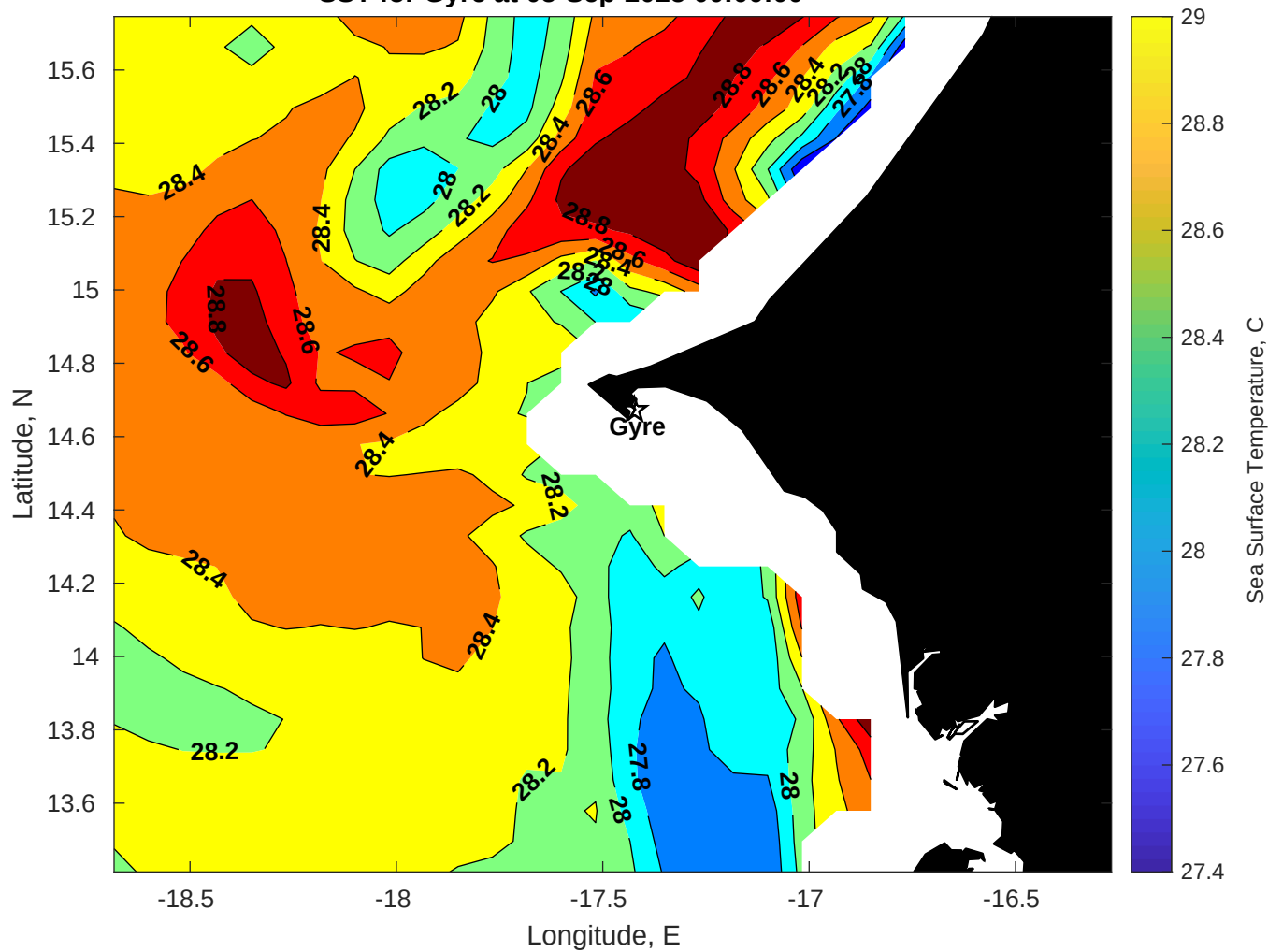
SST for Gyre at 05-Sep-2025 00:00:00
