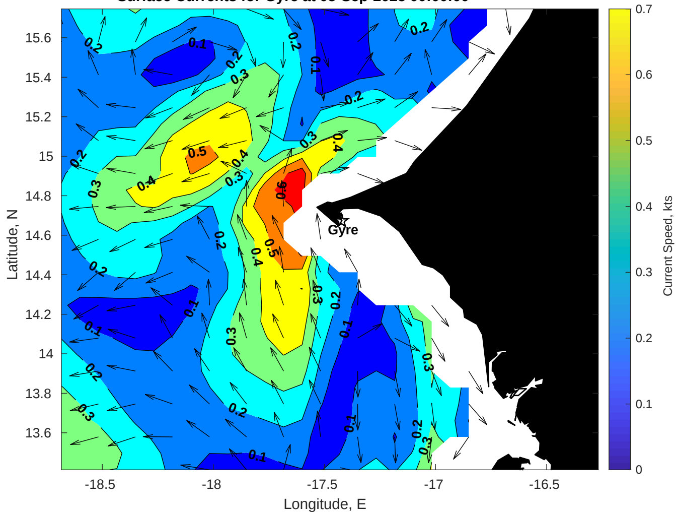
Surface Currents for Gyre at 05-Sep-2025 00:00:00
