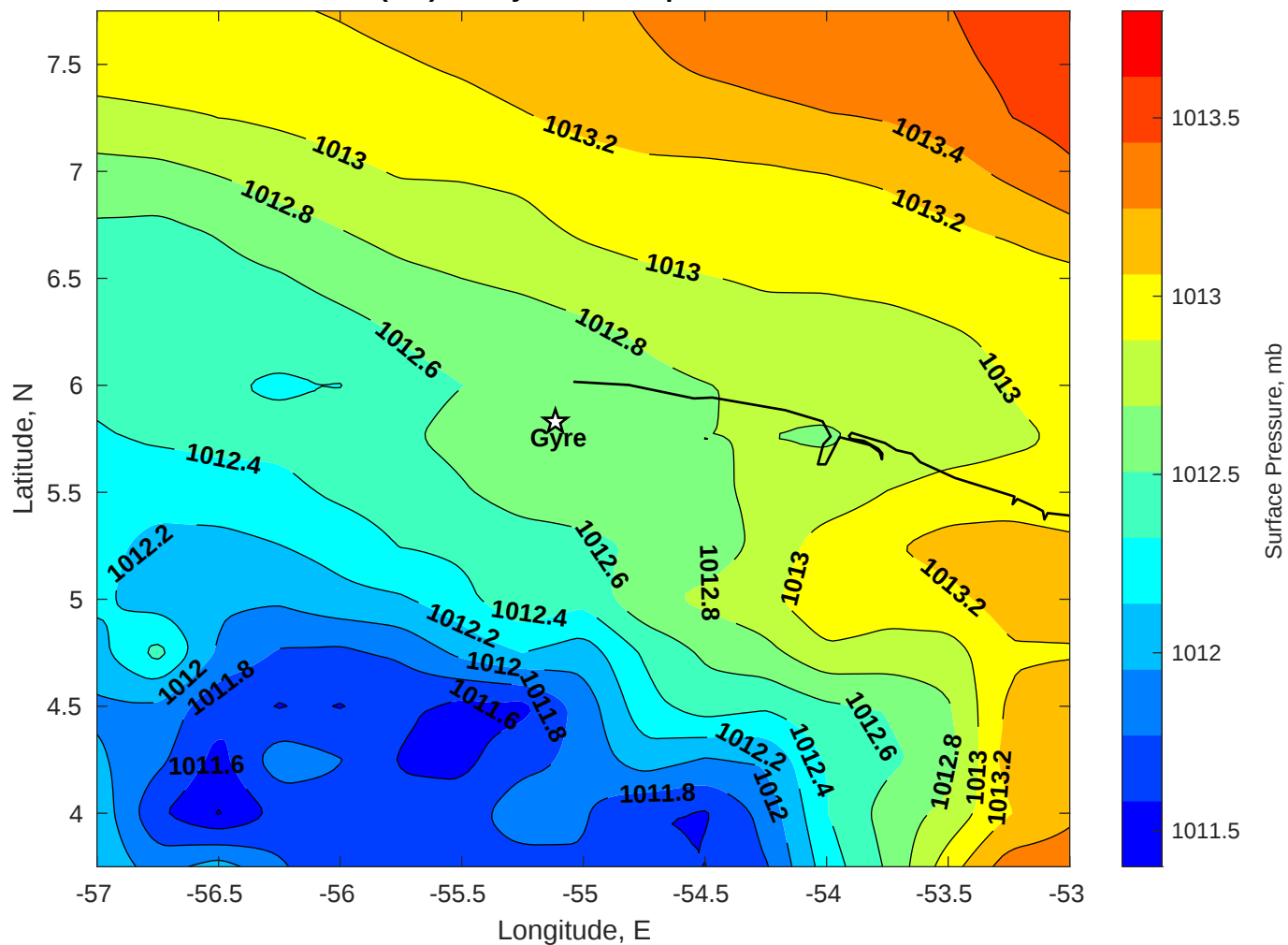
Surface Pressure (mb) for Gyre at 06-Sep-2025 00:00:00
