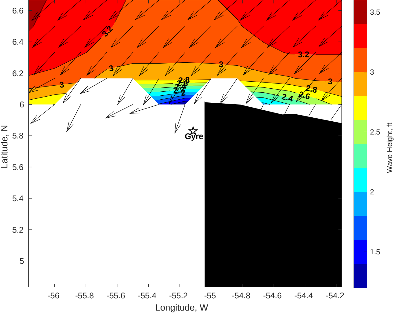
Wave Height (ft) for Gyre at 06-Sep-2025 09:00:00
