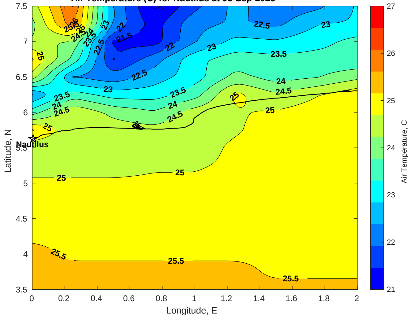
Air Temperature (C) for Nautilus at 06-Sep-2025
