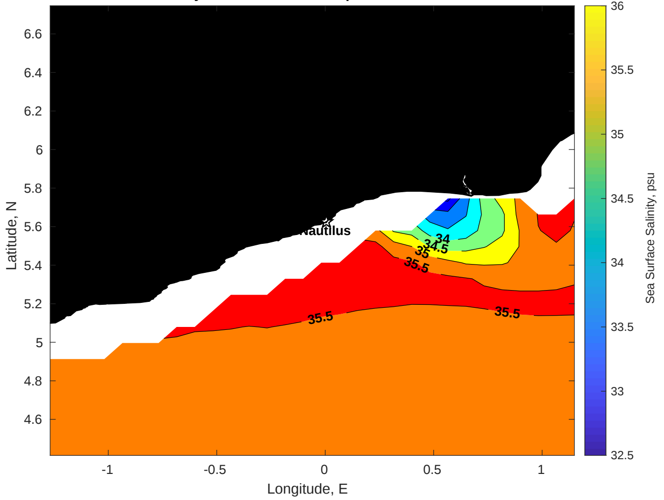
Surface Salinity for Nautilus at 05-Sep-2025 00:00:00
