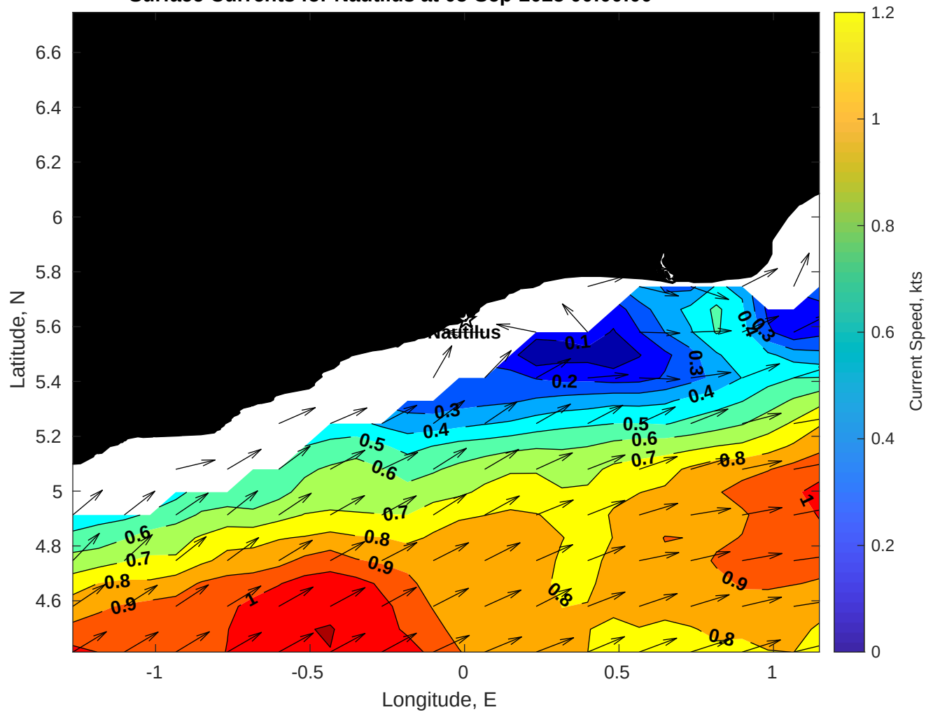
Surface Currents for Nautilus at 05-Sep-2025 00:00:00
