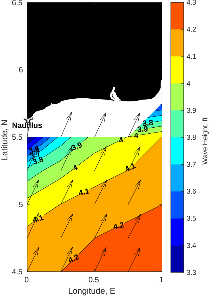
Wave Height (ft) for Nautilus at 06-Sep-2025 09:00:00
