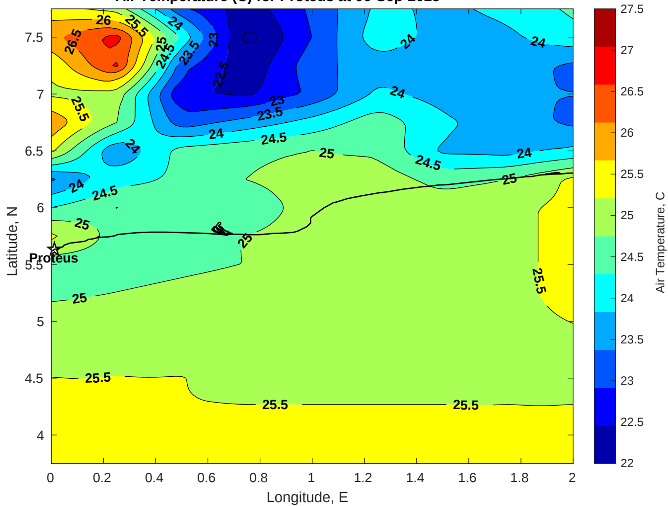
Air Temperature (C) for Proteus at 06-Sep-2025
