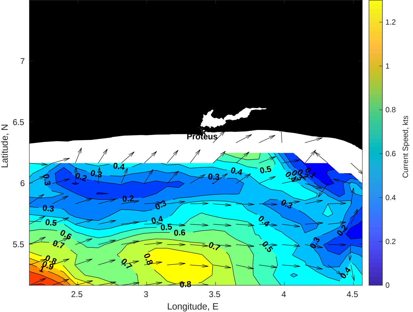
Surface Currents for Proteus at 05-Sep-2025 00:00:00
