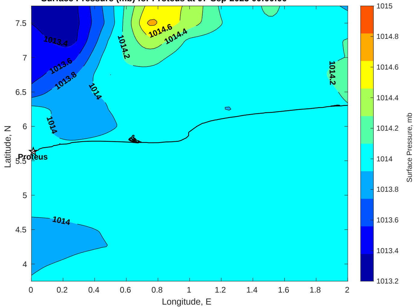
Surface Pressure (mb) for Proteus at 07-Sep-2025 00:00:00
