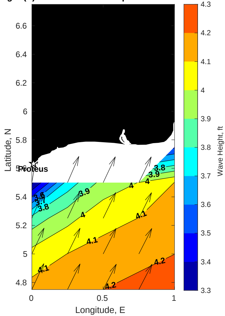
Wave Height (ft) for Proteus at 06-Sep-2025 09:00:00
