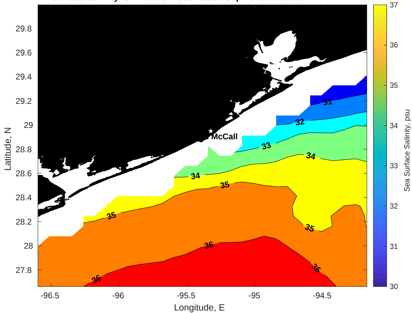
Surface Salinity for Brooks McCall at 06-Sep-2025 00:00:00
