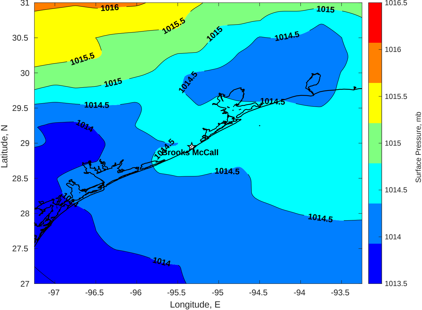
Surface Pressure (mb) for Brooks McCall at 07-Sep-2025 00:00:00
