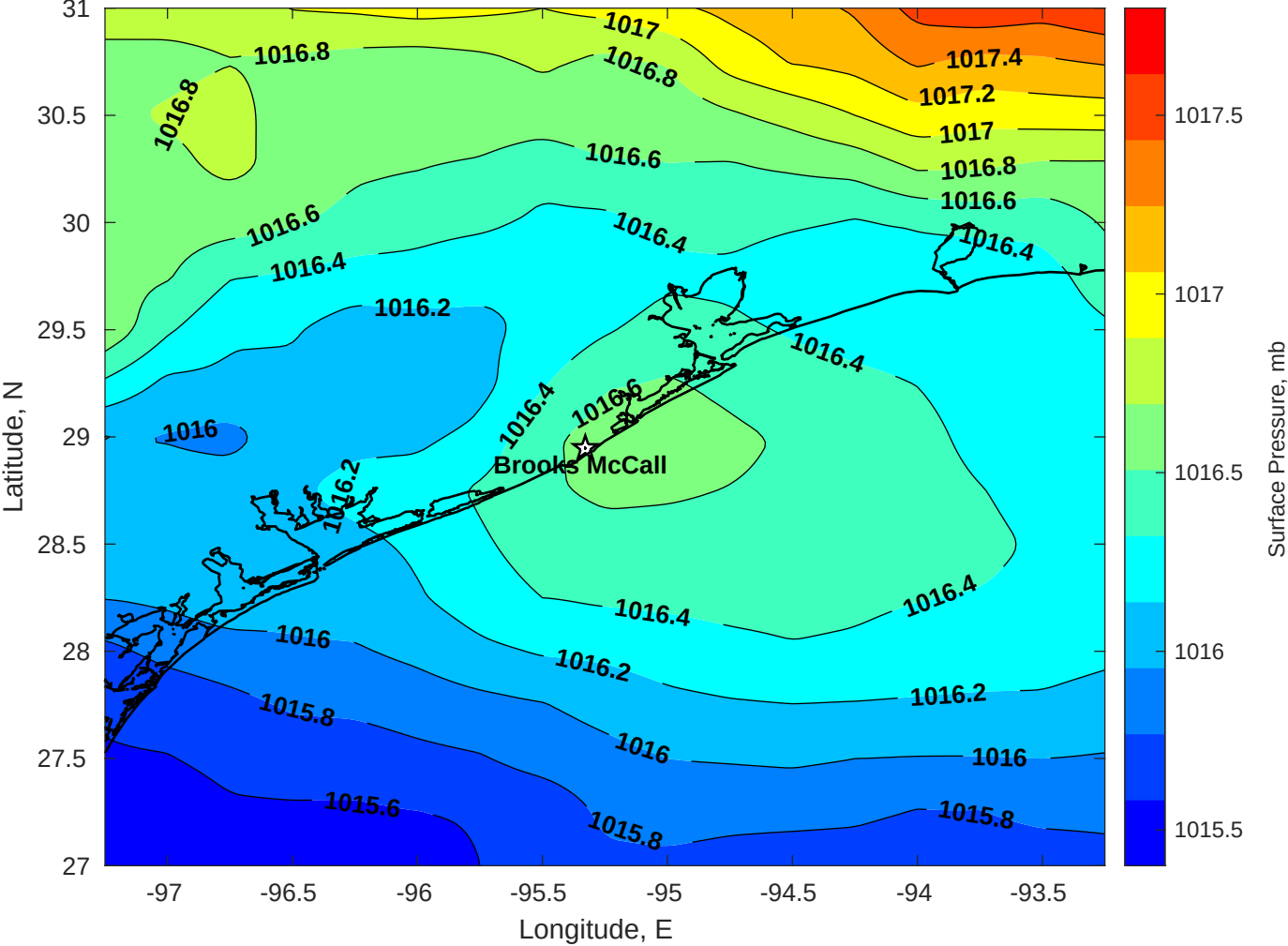
Surface Pressure (mb) for Brooks McCall at 08-Sep-2025 00:00:00
