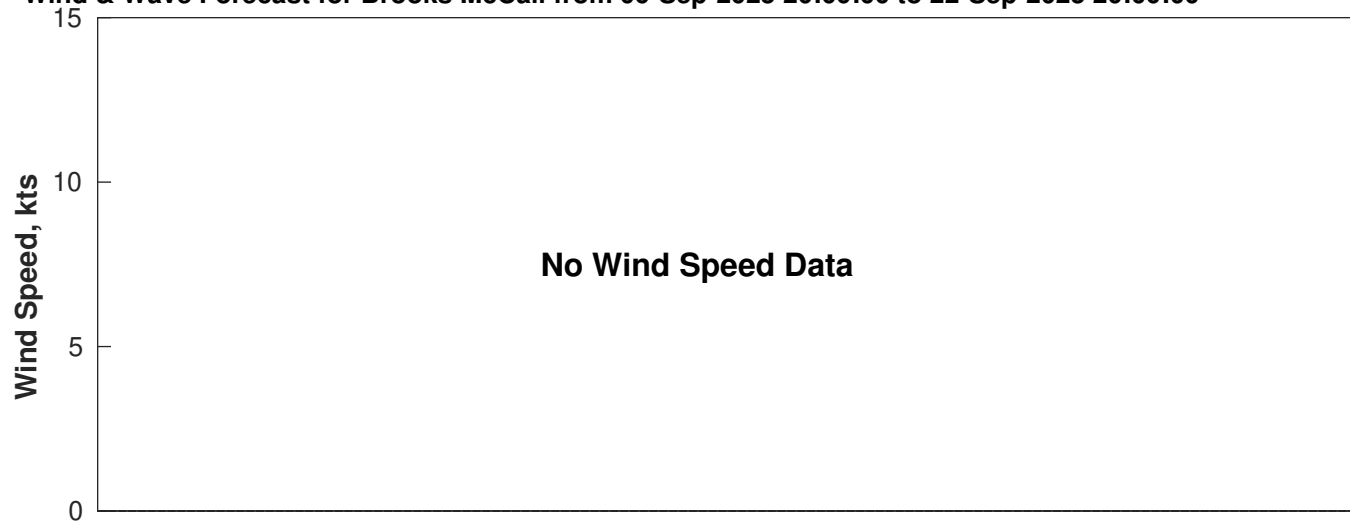
Wind & Wave Forecast for Brooks McCall from 06-Sep-2025 20:00:00 to 22-Sep-2025 20:00:00
