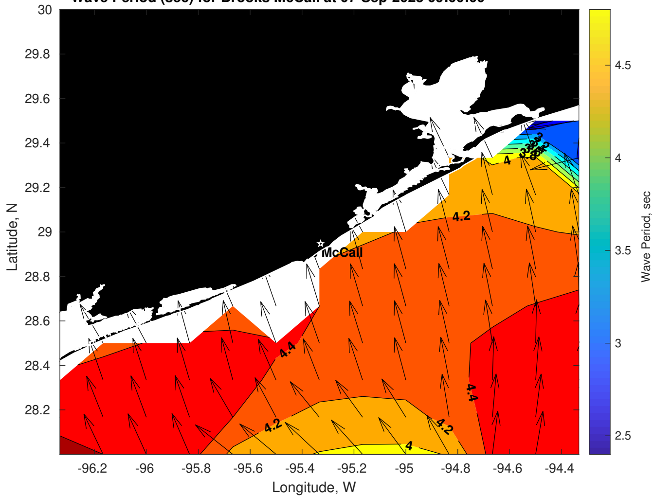
Wave Period (sec) for Brooks McCall at 07-Sep-2025 09:00:00
