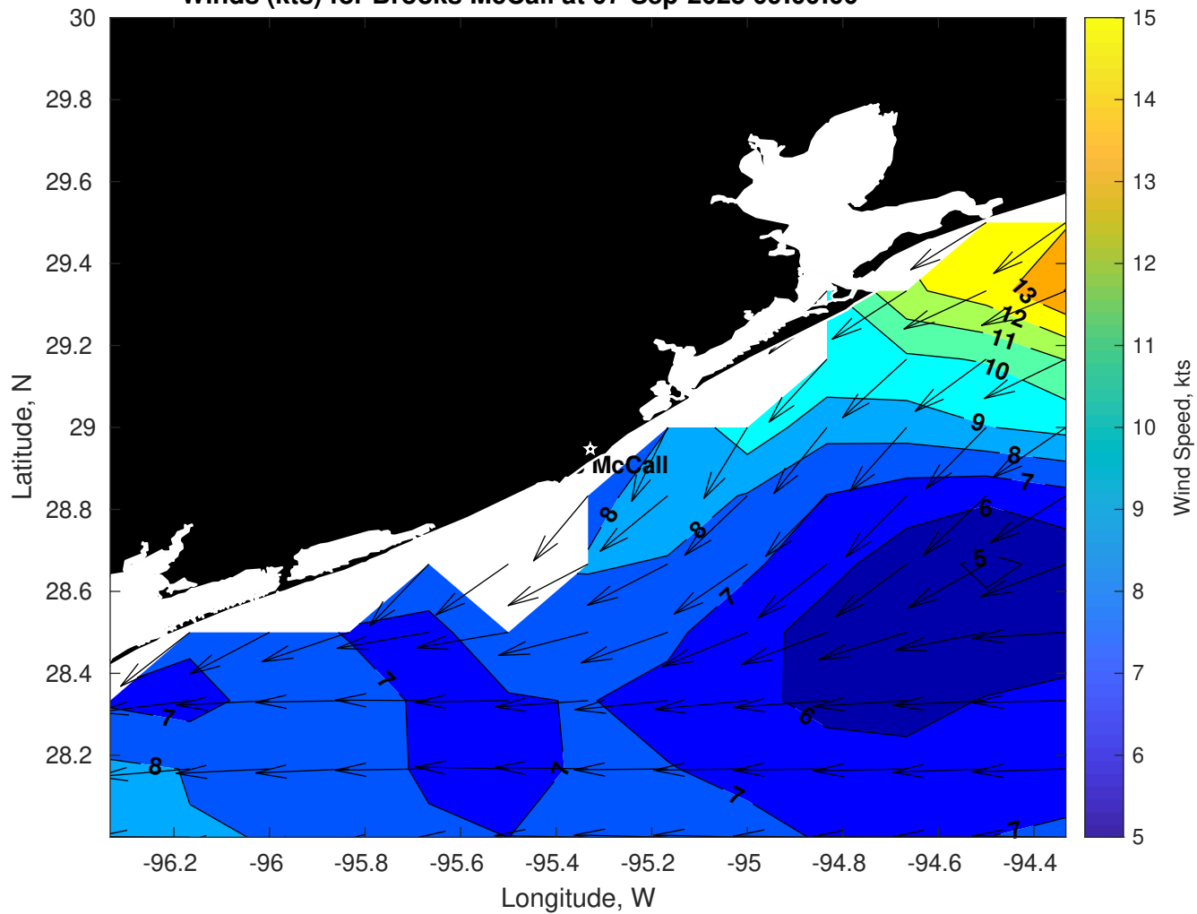
Winds (kts) for Brooks McCall at 07-Sep-2025 09:00:00
