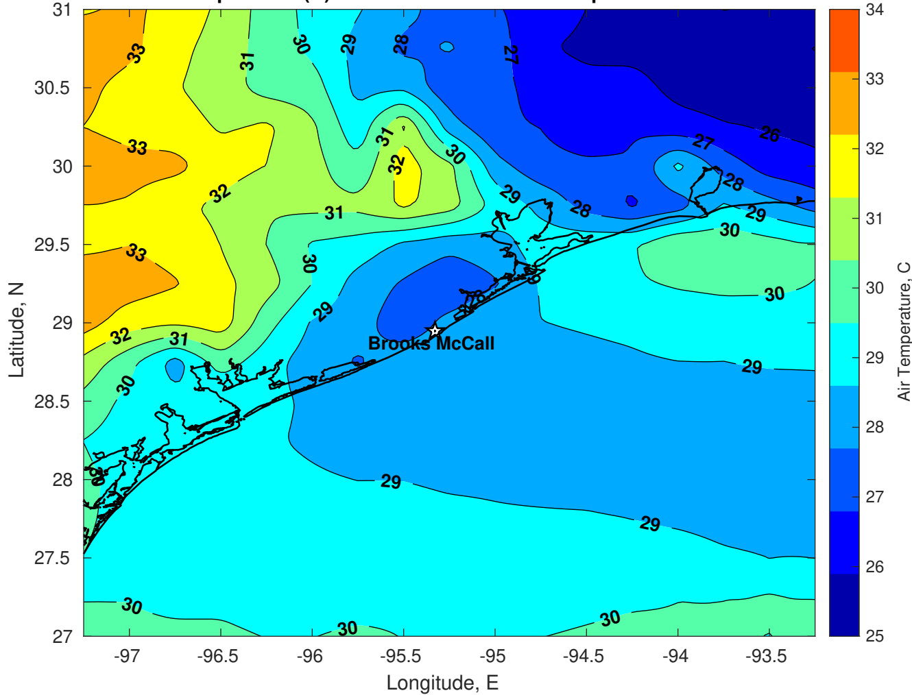
Air Temperature (C) for Brooks McCall at 07-Sep-2025
