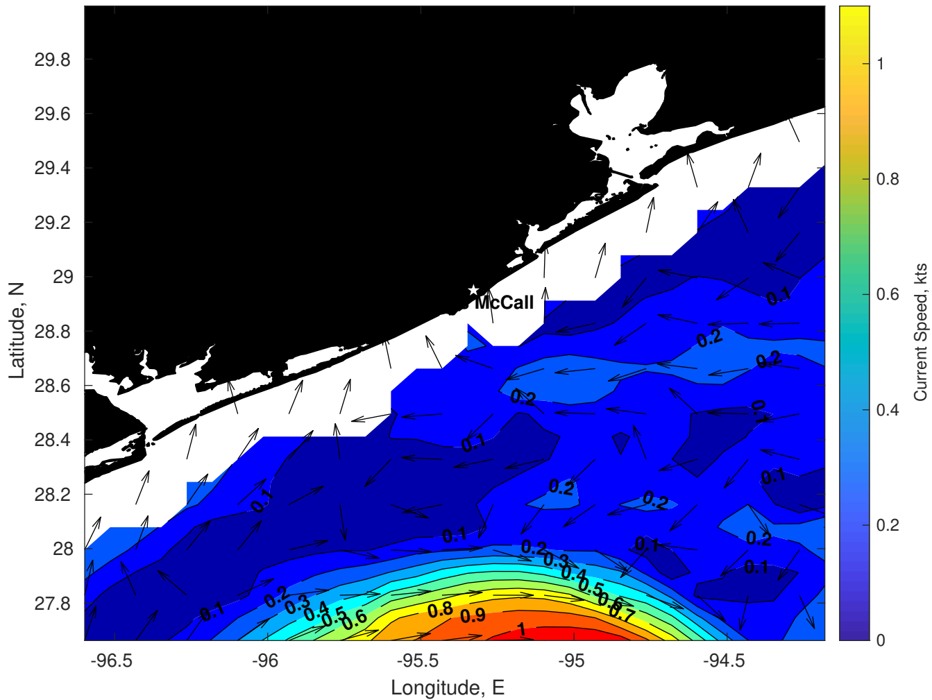
Surface Currents for Brooks McCall at 06-Sep-2025 00:00:00
