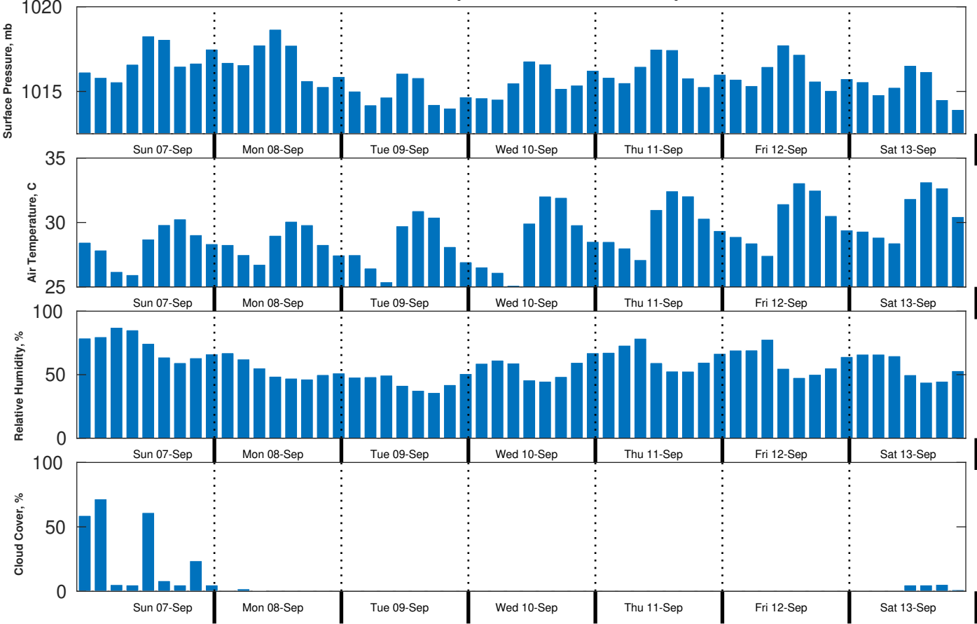
Met Forecast for Brooks McCall from 07-Sep-2025 00:00:00 to 14-Sep-2025 00:00:00
