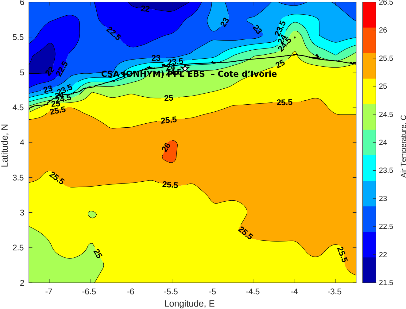
Air Temperature (C) for CSA (ONHYM) PPL EBS - Cote d'Ivoire at 07-Sep-2025
