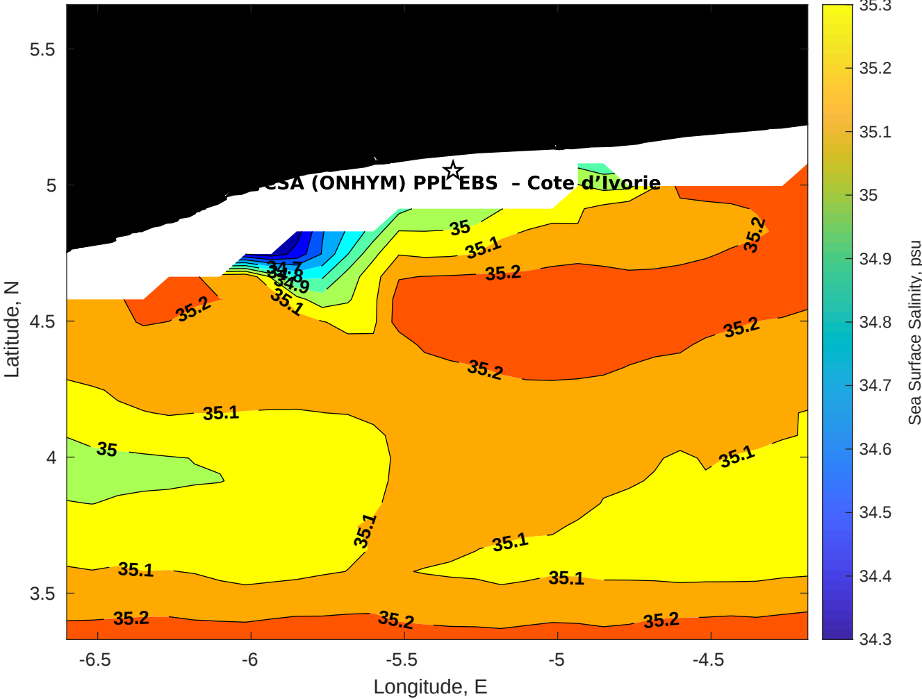
Surface Salinity for CSA (ONHYM) PPL EBS - Cote d'Ivoire at 06-Sep-2025 00:00:00
