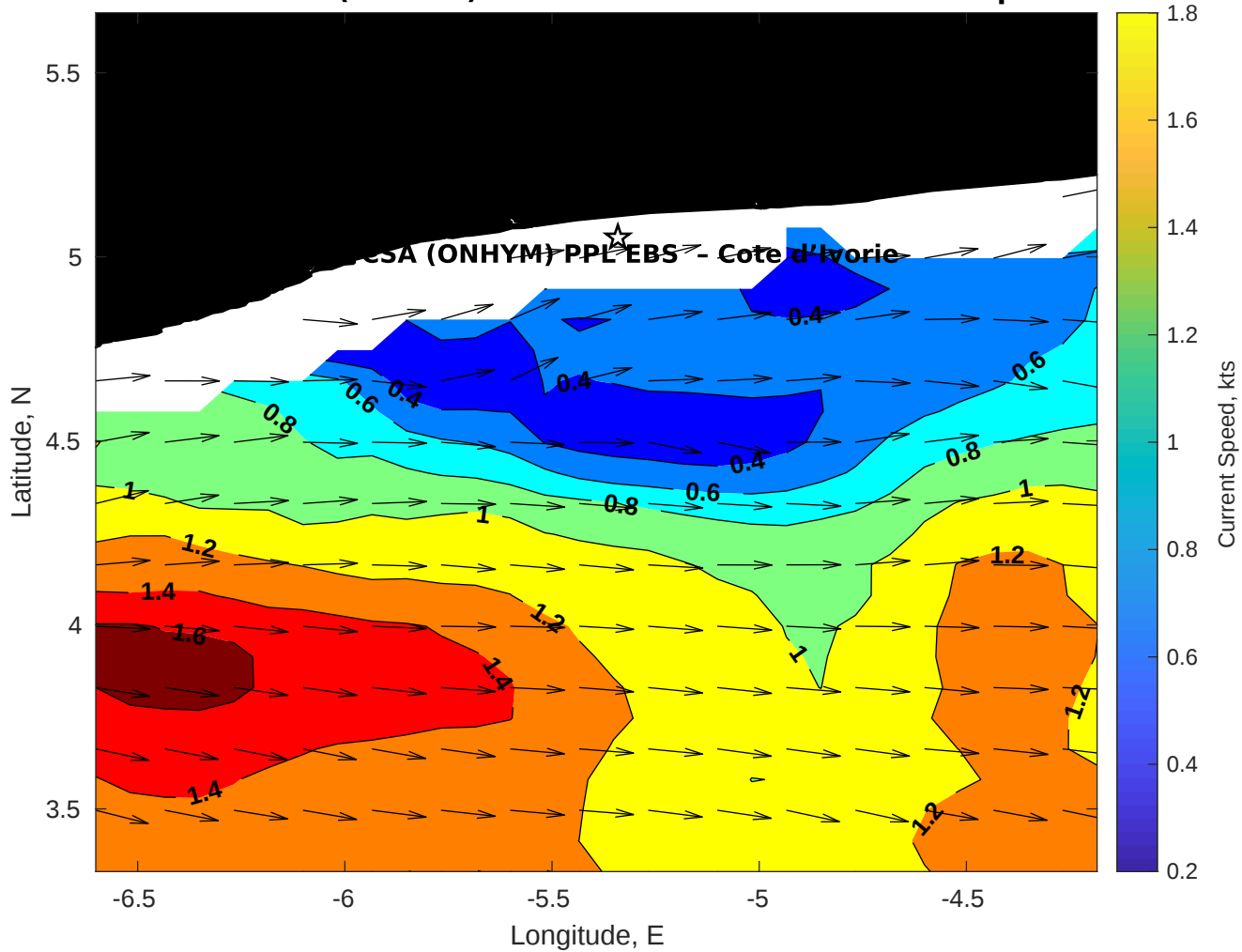
Surface Currents for CSA (ONHYM) PPL EBS - Cote d'Ivoire at 06-Sep-2025 00:00:00
