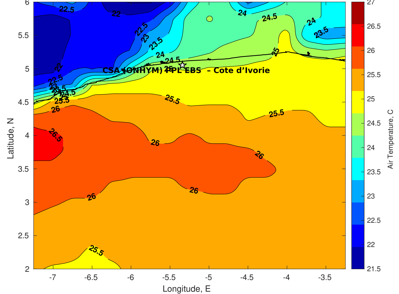
Air Temperature (C) for CSA (ONHYM) PPL EBS - Cote d'Ivoire at 07-Sep-2025
