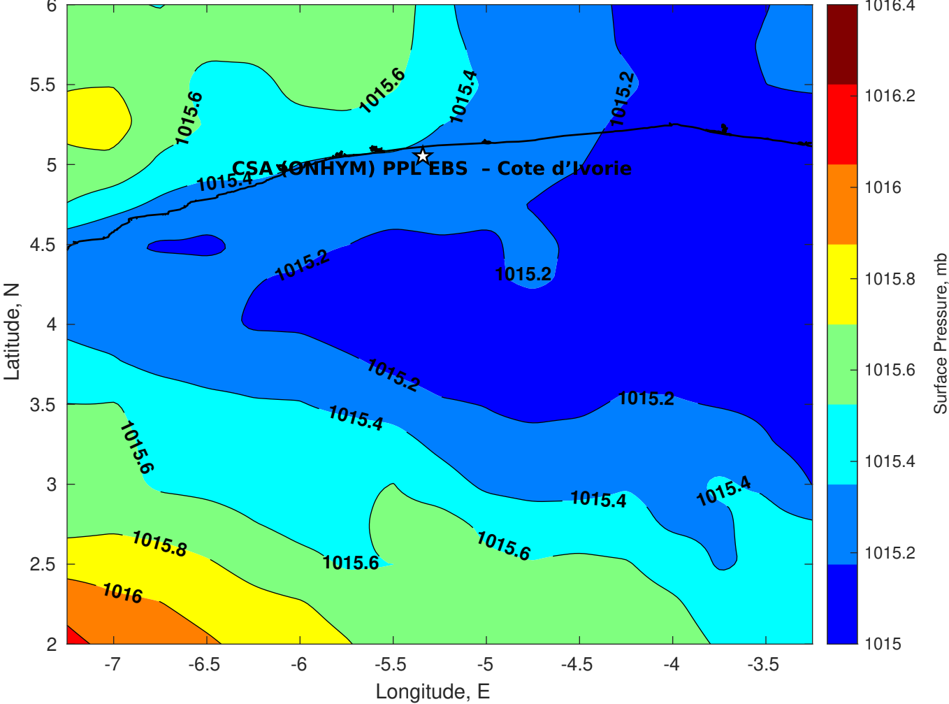
Surface Pressure (mb) for CSA (ONHYM) PPL EBS - Cote d'Ivoire at 09-Sep-2025 00:00:00
