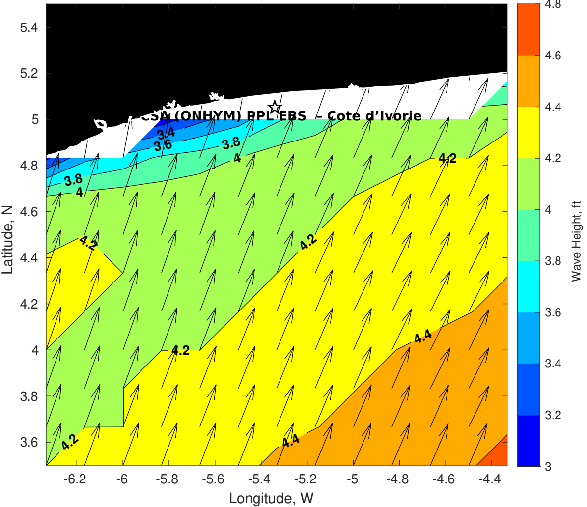
Wave Height (ft) for CSA (ONHYM) PPL EBS - Cote d'Ivoire at 07-Sep-2025 09:00:00
