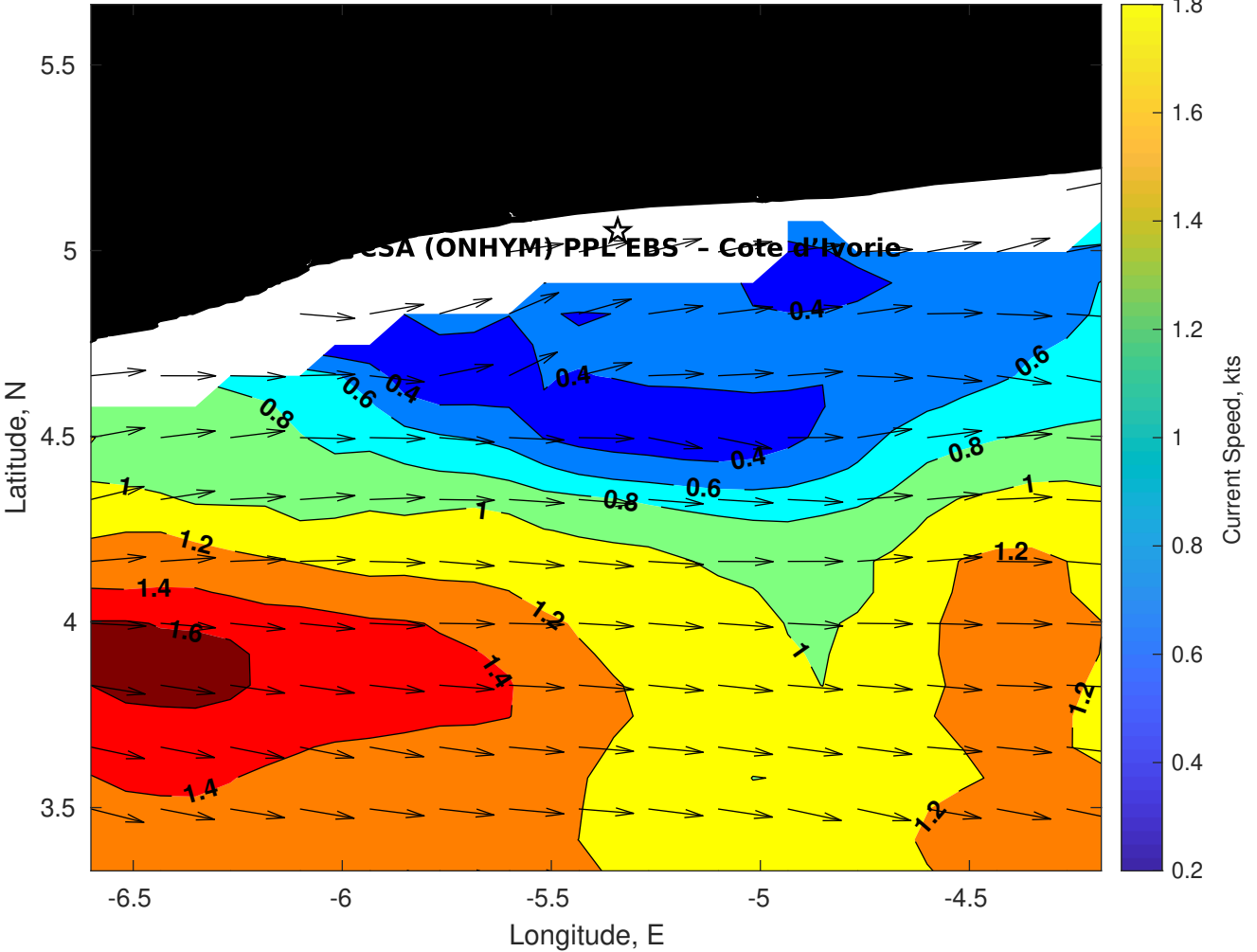
Surface Currents for CSA (ONHYM) PPL EBS - Cote d'Ivoire at 06-Sep-2025 00:00:00
