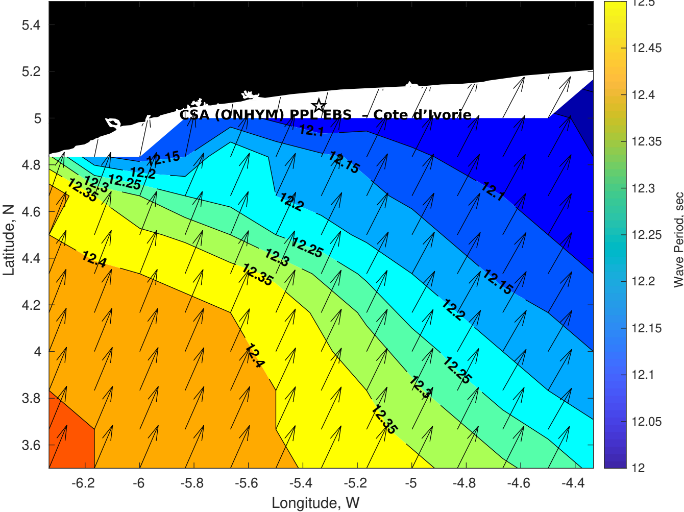
Wave Period (sec) for CSA (ONHYM) PPL EBS - Cote d'Ivoire at 07-Sep-2025 09:00:00
