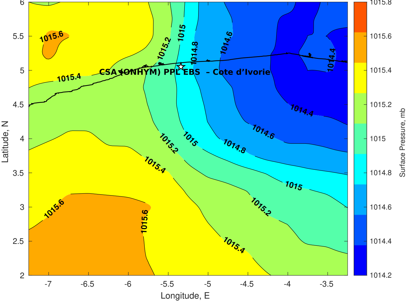
Surface Pressure (mb) for CSA (ONHYM) PPL EBS - Cote d'Ivoire at 07-Sep-2025 00:00:00
