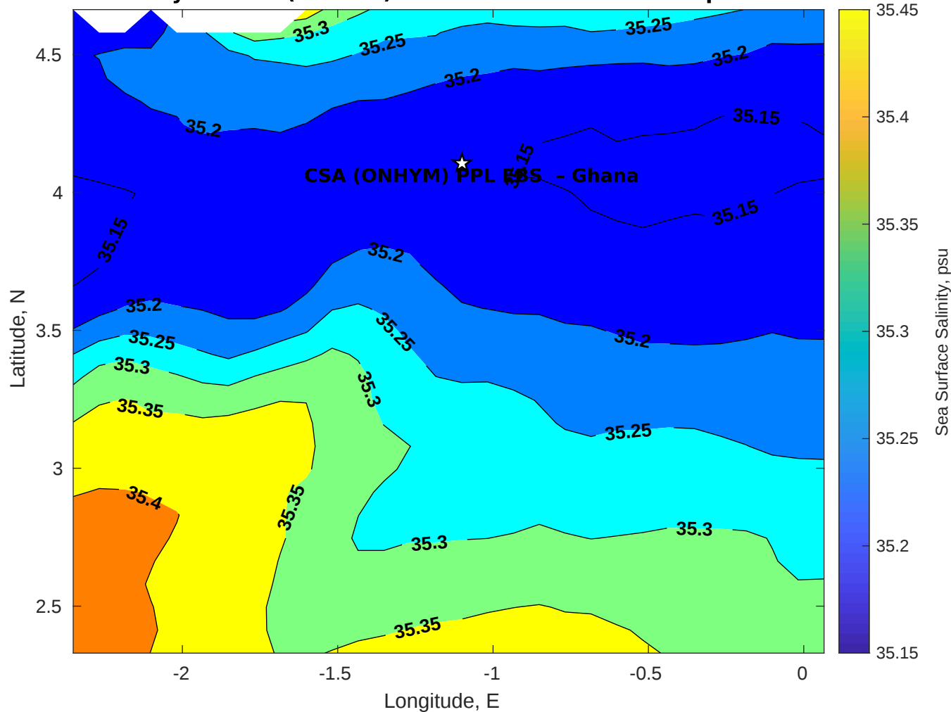
Surface Salinity for CSA (ONHYM) PPL EBS - Ghana at 06-Sep-2025 00:00:00
