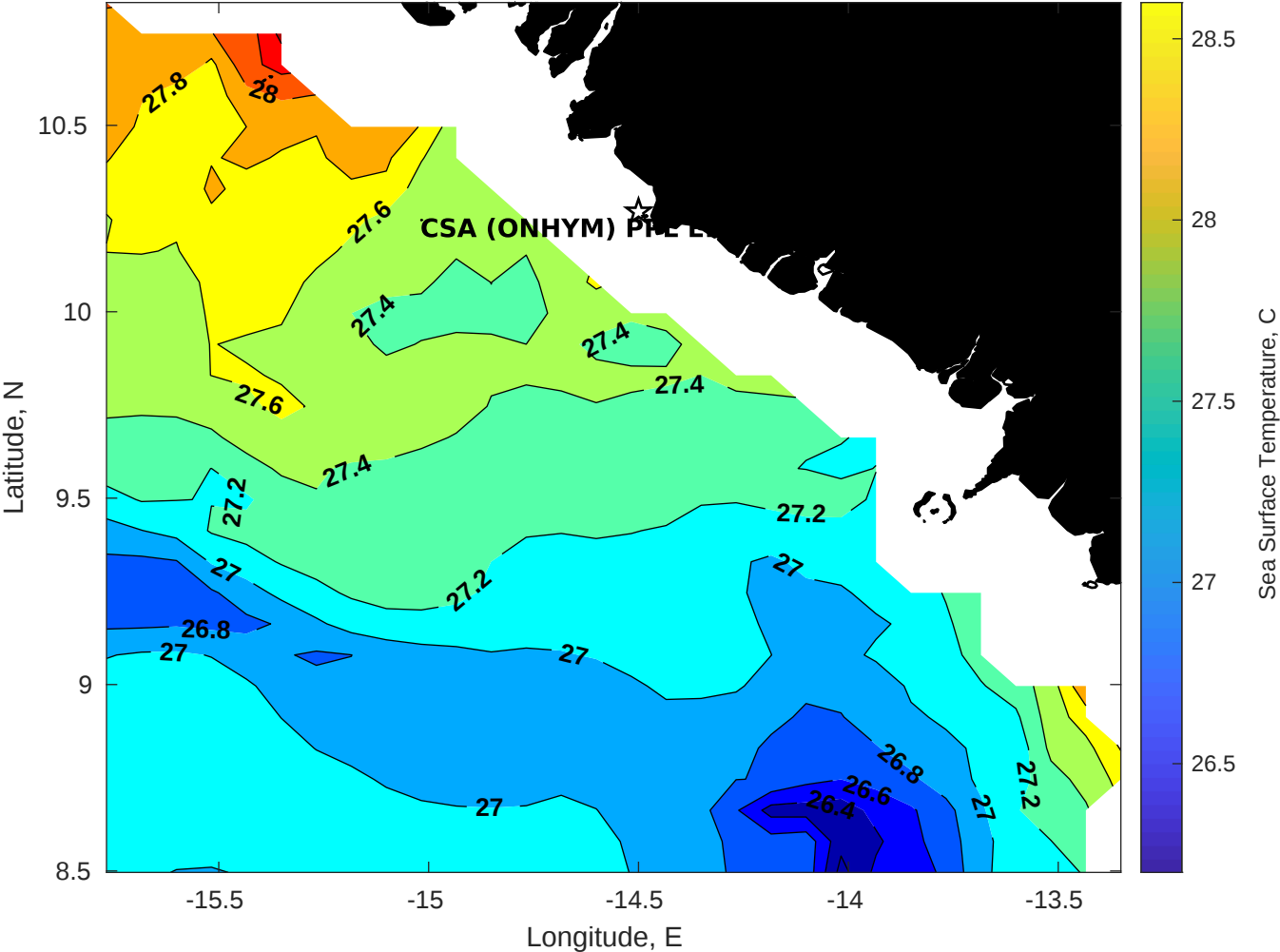
SST for CSA (ONHYM) PPL EBS - Guinea at 06-Sep-2025 00:00:00
