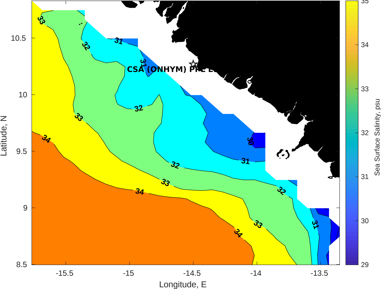
Surface Salinity for CSA (ONHYM) PPL EBS - Guinea at 06-Sep-2025 00:00:00
