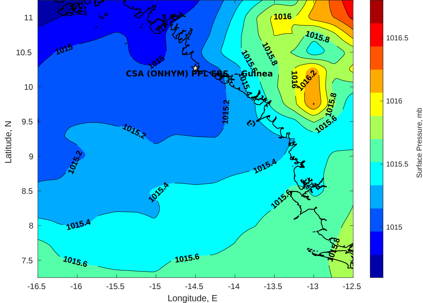
Surface Pressure (mb) for CSA (ONHYM) PPL EBS - Guinea at 08-Sep-2025 00:00:00
