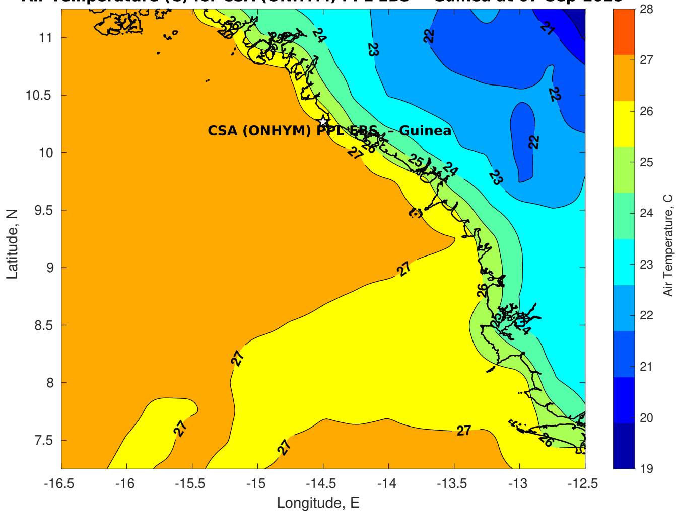
Air Temperature (C) for CSA (ONHYM) PPL EBS - Guinea at 07-Sep-2025
