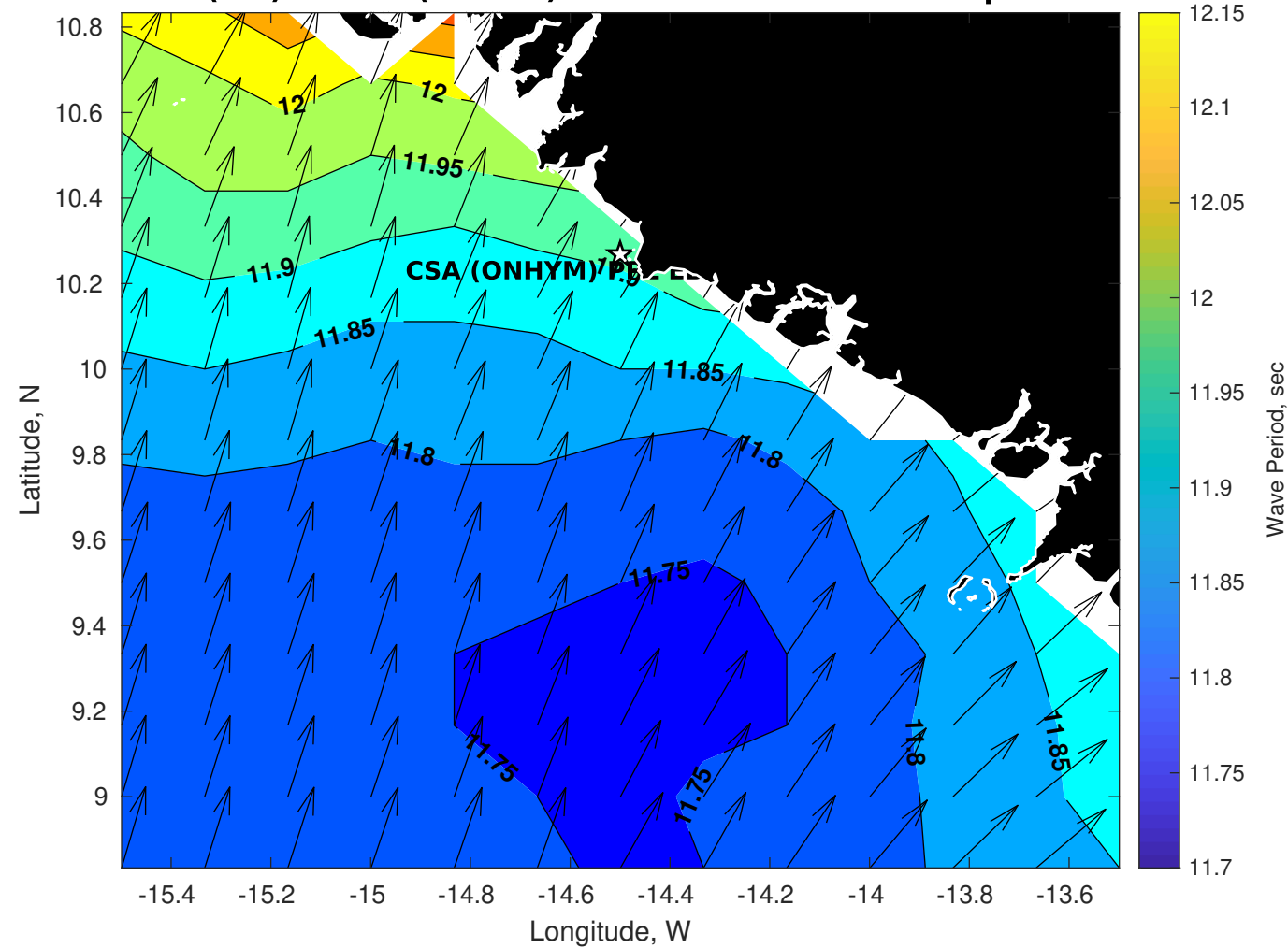
Wave Period (sec) for CSA (ONHYM) PPL EBS - Guinea at 07-Sep-2025 09:00:00
