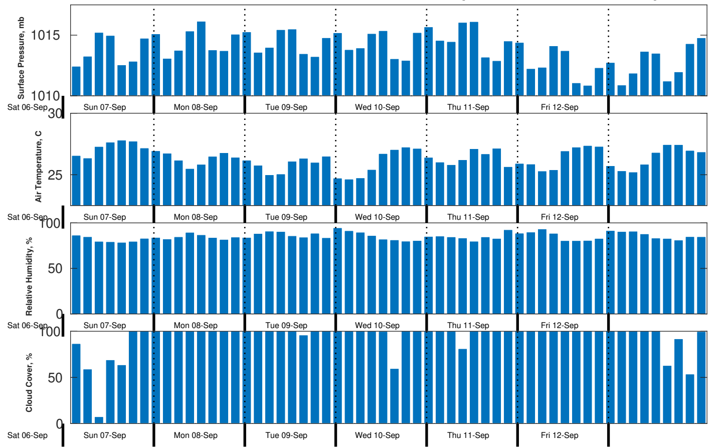
Met Forecast for CSA (ONHYM) PPL EBS - Guinea from 07-Sep-2025 00:00:00 to 14-Sep-2025 00:00:00
