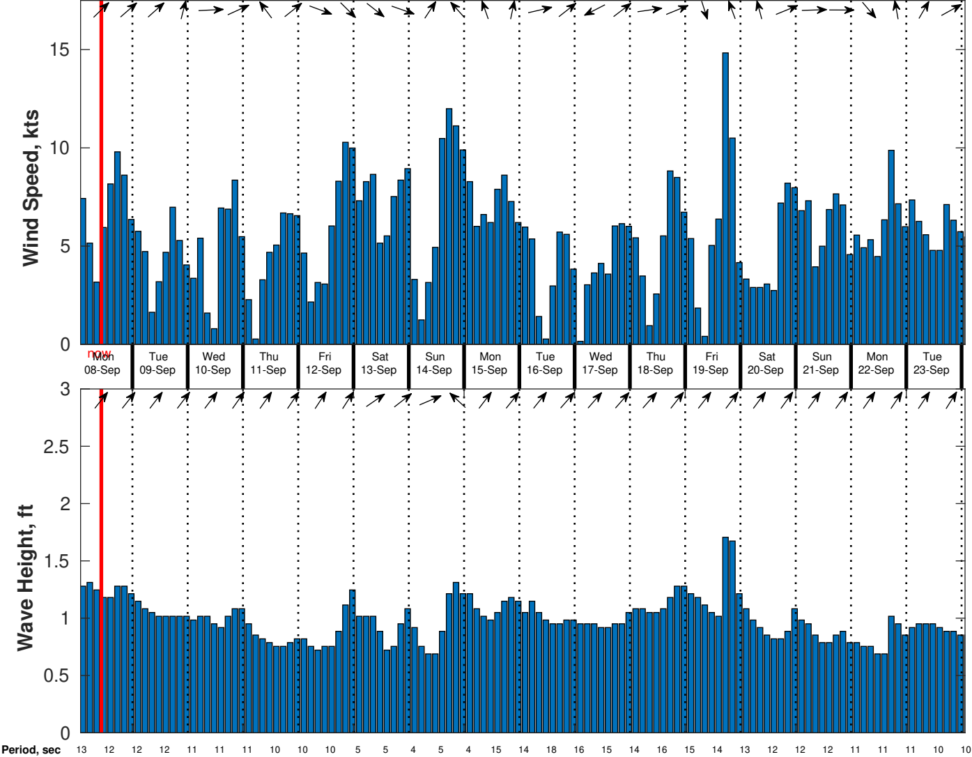
Wind & Wave Forecast for CSA (ONHYM) PPL EBS - Guinea from 07-Sep-2025 01:00:00 to 23-Sep-2025 01:00:00
