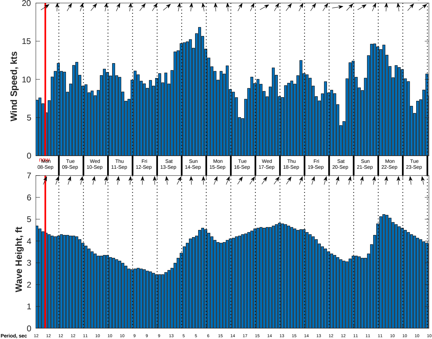
Wind & Wave Forecast for CSA (ONHYM) PPL EBS - Liberia from 07-Sep-2025 01:00:00 to 23-Sep-2025 01:00:00
