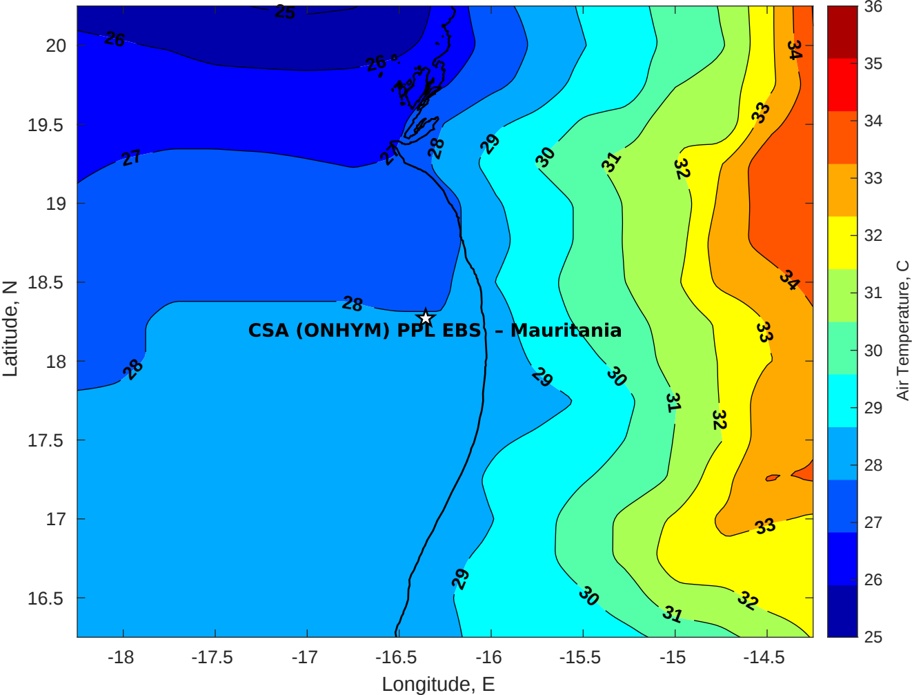
Air Temperature (C) for CSA (ONHYM) PPL EBS - Mauritania at 07-Sep-2025
