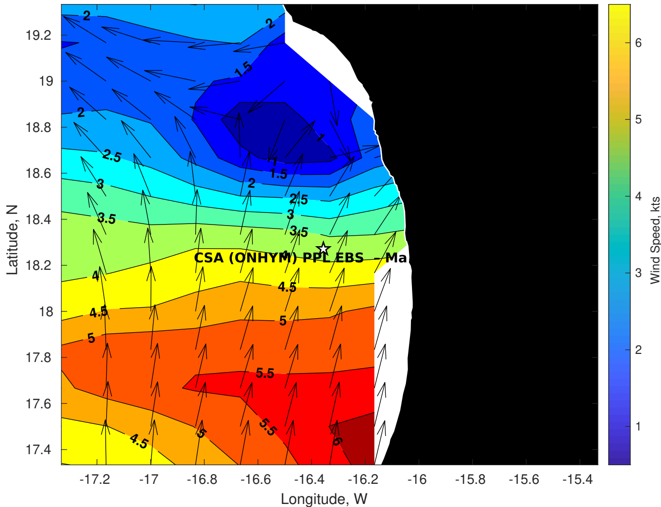
Winds (kts) for CSA (ONHYM) PPL EBS - Mauritania at 07-Sep-2025 09:00:00
