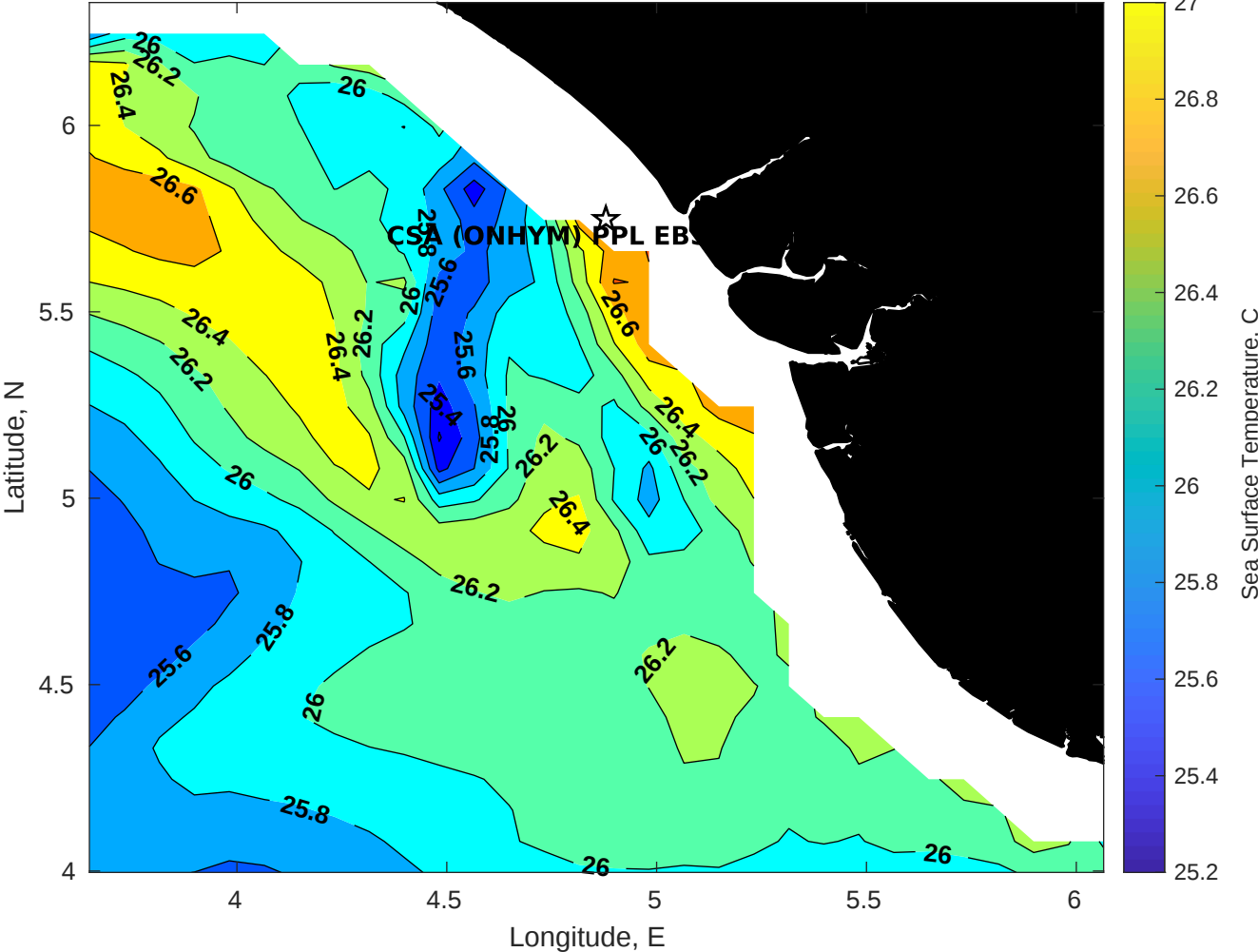
SST for CSA (ONHYM) PPL EBS - Nigeria at 06-Sep-2025 00:00:00
