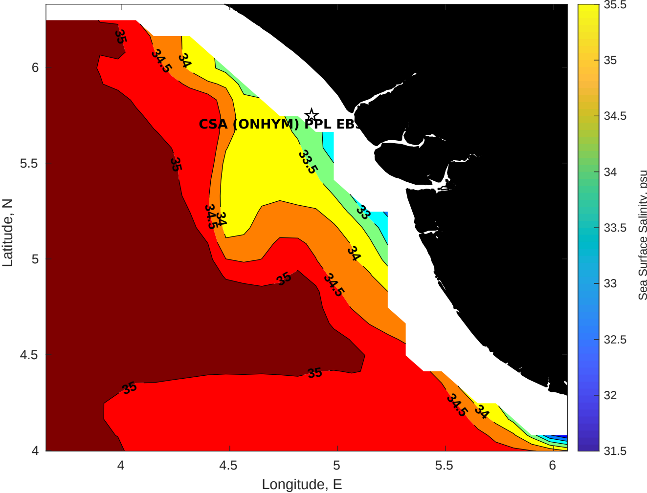
Surface Salinity for CSA (ONHYM) PPL EBS - Nigeria at 06-Sep-2025 00:00:00
