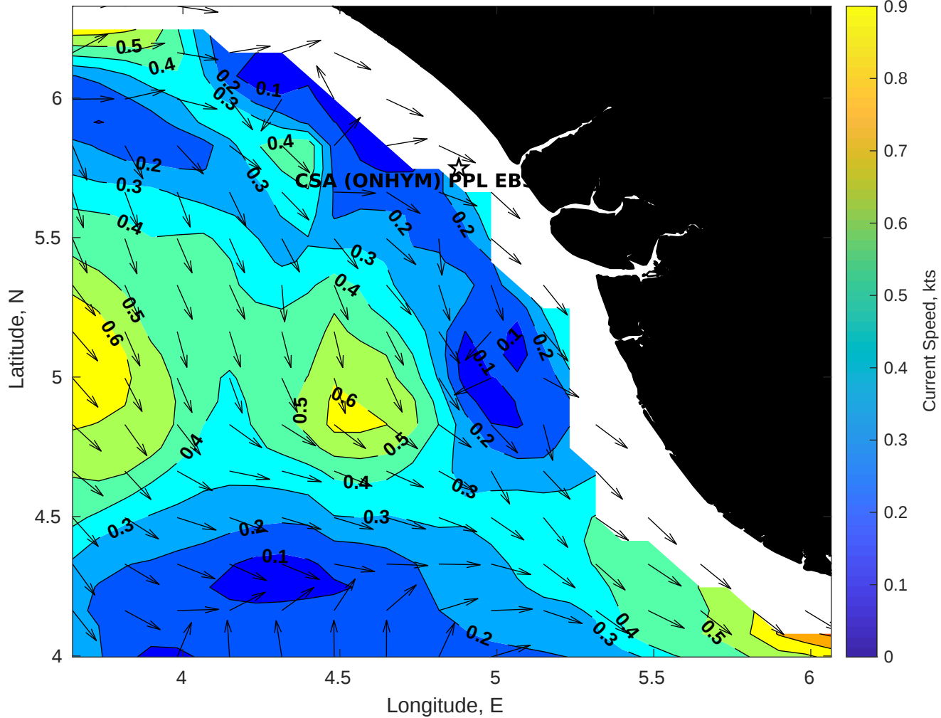
Surface Currents for CSA (ONHYM) PPL EBS - Nigeria at 06-Sep-2025 00:00:00
