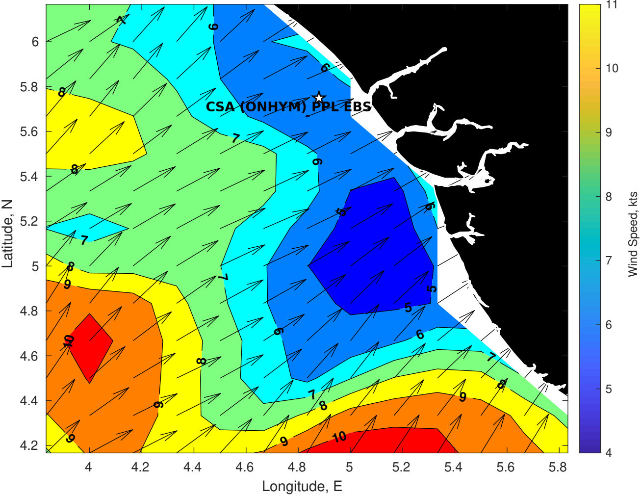
Winds (kts) for CSA (ONHYM) PPL EBS - Nigeria at 07-Sep-2025 09:00:00
