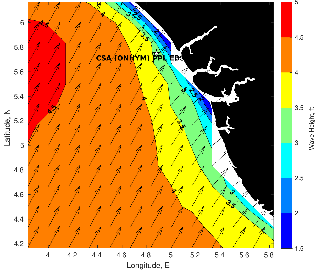
Wave Height (ft) for CSA (ONHYM) PPL EBS - Nigeria at 07-Sep-2025 09:00:00
