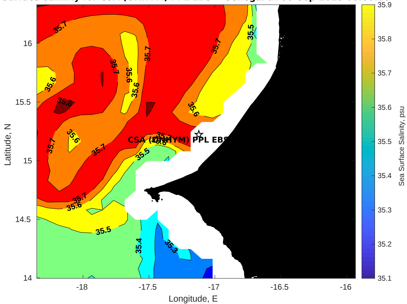
Surface Salinity for CSA (ONHYM) PPL EBS - Senegal at 06-Sep-2025 00:00:00
