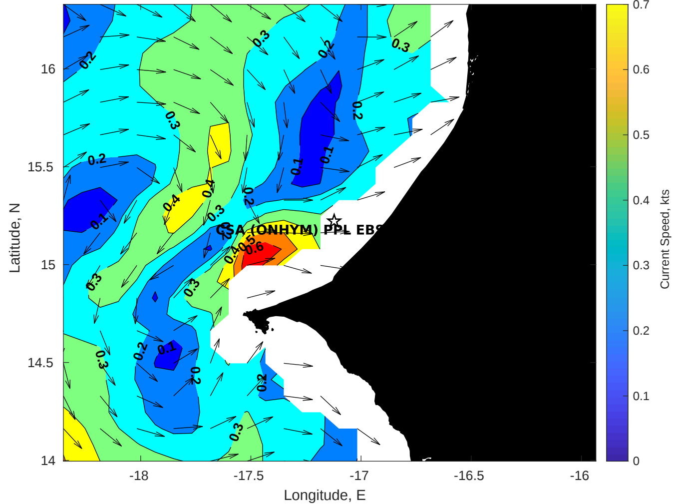
Surface Currents for CSA (ONHYM) PPL EBS - Senegal at 06-Sep-2025 00:00:00
