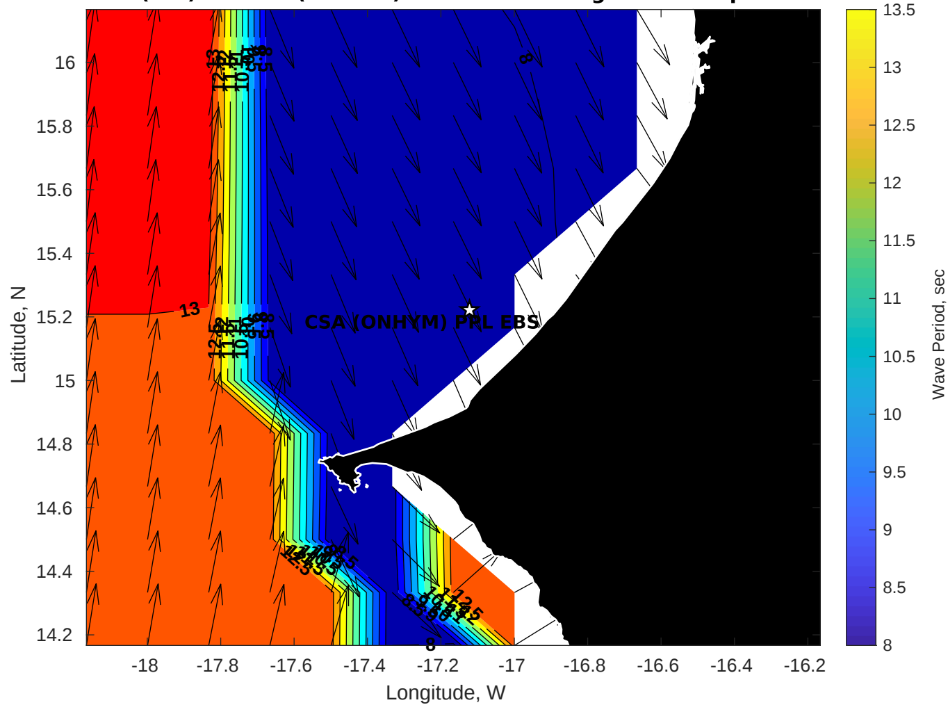
Wave Period (sec) for CSA (ONHYM) PPL EBS - Senegal at 07-Sep-2025 09:00:00
