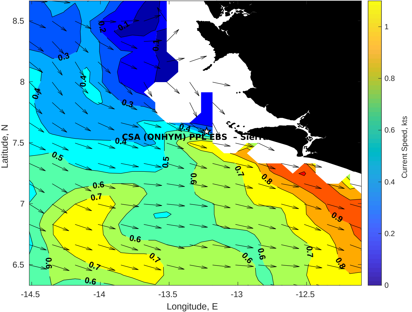
Surface Currents for CSA (ONHYM) PPL EBS - Sierra Leone at 06-Sep-2025 00:00:00
